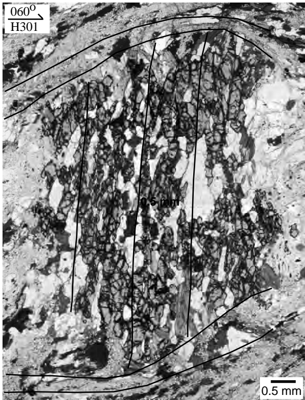
FIGURE 5. Garnet porphyroblast with inclusion trails truncated completely by the matrix foliation. The foliation in the matrix, which truncates the inclusion trails in the porphyroblast, has been partially sericitized post foliation development as the tiny muscovite grains have random orientations. This has not affected the inclusion trail geometry or the matrix foliation geometry. Plane polarized light. FIA trends 135^\circ . Vertical section with strike shown by horizontal, single-barbed arrow. (Sample H301 located in Fig. 12.)
