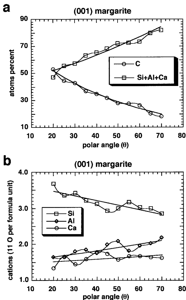
FIGURE 3. Relative concentration vs. polar angle ( \theta ). (a) The relationship between C relative concentration and polar angle clearly proves that C is limited to the top most part of the surface. The lack of diffraction modulation suggests that C is amorphous. (b) The crystal termination is probably made up of Si. The Ca peak at 25^\circ \theta may not be relevant. The cubic spline (light line) and exponential curve (heavy line) fits are also given.
