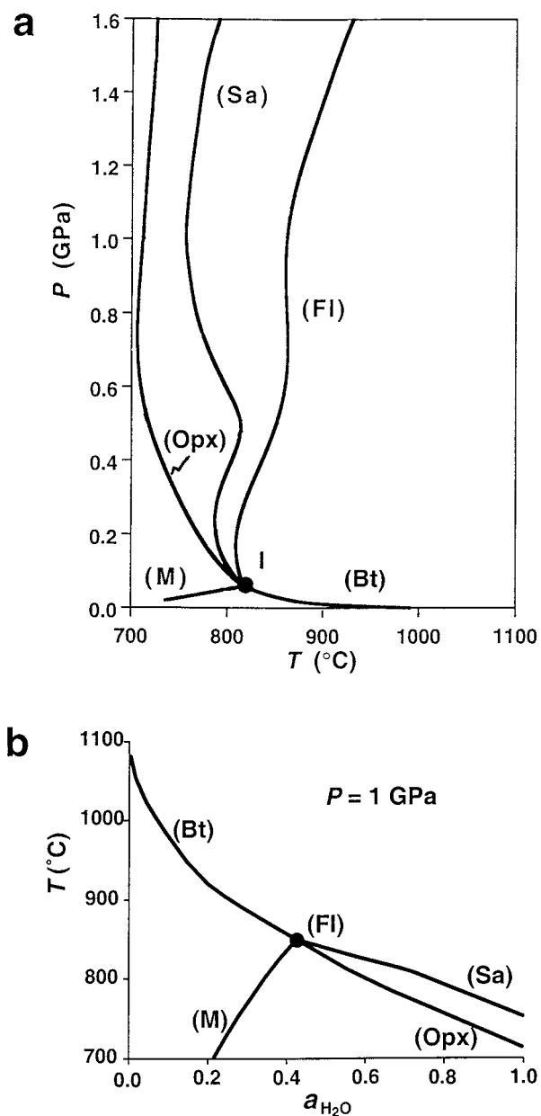
FIGURE 5. (a) P - T and (b) isobaric T - a_{\text{H}_2\text{O}} sections through the quartz-saturated portion of the system \text{KAlO}_2 - \text{MgO} - \text{FeO} - \text{SiO}_2 - \text{H}_2\text{O} , for X_{\text{Fe}} = 0 , based on the work of Vielzeuf and Clemens (1992), Clemens (1995), and Clemens et al. (1997), showing the univariant equilibria surrounding the invariant point (I), involving the phases Bt, Opx, Sa, Qtz, M, and Fl. The equilibria (labeled according to the absent phase) are:
