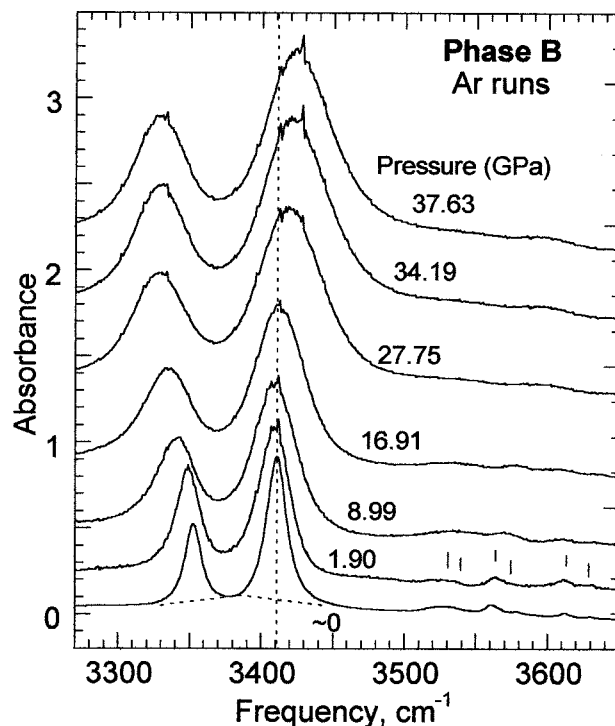
FIGURE 6. Representative near-IR spectra of OH in phase B from "dry" Ar runs obtained during decompression. Vertical dashes on the 1.9 GPa spectrum indicate trace H in structural defects. The dotted lines on the ~0 GPa spectrum indicate the baselines used in determining peak widths and heights and starting and ending points to obtain areas from integration. Because the ~0 GPa spectrum was collected without a gasket and before compression, its intensity corresponds only roughly with the pressure series. Each spectrum above 1 atm was offset sequentially by 0.4 absorbance units for clarity. The vertical dotted line serves to indicate the initial decrease in \nu for both strong bands.
