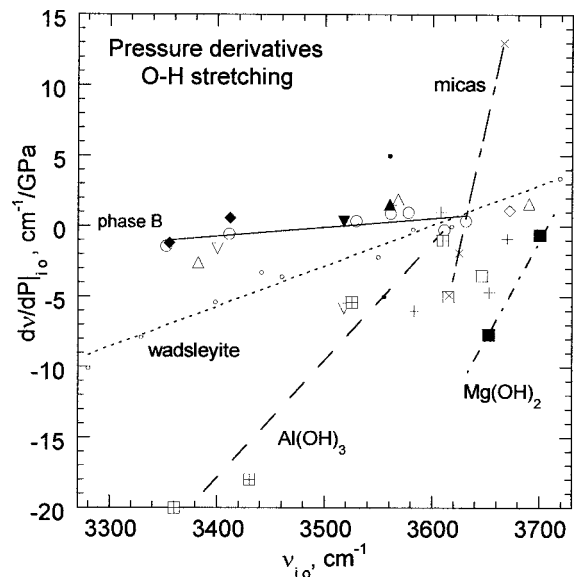
FIGURE 12. Correlation of the pressure response dv/dP with \nu for the OH bands of hydrous phases. Various lines show linear least-squares fits of OH within a given mineral. Micas were plotted together. The trend for phase B (solid line) also fits the other DHMS. Small open circle = wadsleyite IR (Cynn and Hofmeister 1994). Large open circle = phase B IR (this work). Filled diamond = shyB Raman (this work). Filled downward-pointing triangle = phase A Raman (this work). Open downward-pointing triangle = phase A Raman (Liu et al. 1997a). Filled upward-pointing triangle = chondrodite Raman (this work). Open upward-pointing triangle = chondrodite IR (Williams 1992). Open square = portlandite \text{Ca}(\text{OH})_2 Raman and IR (Meade et al. 1992). Filled square = brucite \text{Mg}(\text{OH})_2 Raman (Duffy et al. 1995) and IR (Kruger et al. 1989). Square with cross = approximate slopes for gibbsite \text{Al}(\text{OH})_3 Raman (Huang et al. 1996). Open diamond = talc Raman (Holtz et al. 1993). X = mica Raman (Holtz et al. 1993). Small filled circle = analcime Raman (Velde and Besson 1980). For the latter, pressure is probably not accurate. + = OH in the Si site of garnet (Knittle et al. 1992).
