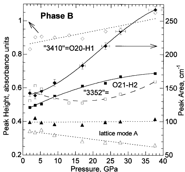
FIGURE 8. Peak areas and heights of major near-IR peaks in phase B during decompression in Ar. Data were not collected for this series at 1 atm. Least-squares fits and error bars are shown. Dashed lines, linear fits. Solid lines polynomial fits. Open symbols maximum absorbance (left-hand scale pertains) and filled symbols area obtained by integrating (right-hand scale pertains). Diamonds the peak initially at 3410.7\text{ cm}^{-1} ; squares the peak initially at 3352\text{ cm}^{-1} .
