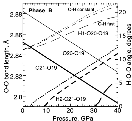
FIGURE 11. Dependence of bond parameters involving hydroxyl in phase B on pressure, calculated from the frequencies and O-O bond lengths at 1 atm. Heavy lines, shorter O-O bond involving H2. Light lines, longer O-O bond involving H1. Solid lines, O-O19 distances. Dotted lines, calculated assuming that the O-H distance is unchanged. Dashed lines, calculated assuming that the rate of change of trace hydroxyl applies to the stoichiometric sites. Long dashed lines, rate of change of O-H is four times that of the trace hydroxyl. For H2, the angle is 0° until a minimum pressure is reached. See text for details and Figure 10 for the hydroxyl configuration.
