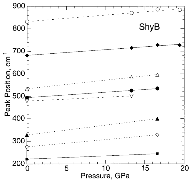
FIGURE 4. Dependence of Raman lattice modes of shyB on pressure. All lines are linear least-squares fits. Only the intense peaks could be traced reliably; hence data points at low frequency are fewer in number.
