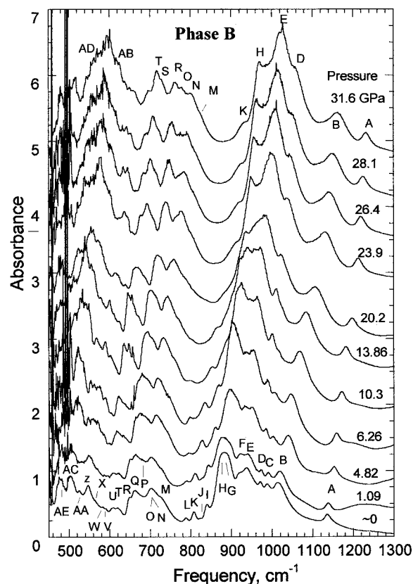
FIGURE 1. Selected mid-IR spectra of phase B from the \text{N}_2 runs. Lattice modes are labeled alphabetically with reference to Table 2. Pressures are given on the right hand side. Each spectrum above 1 atm was offset sequentially by increments of 0.5 absorbance units for clarity.
