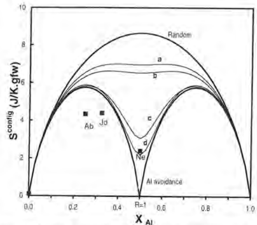
FIGURE 12. Configurational entropy of Na-aluminosilicate glasses at T = 1000 K. S^{\text{config}} was calculated from (a) Equation 15 with Q = 0.85 ; (b) Equation 14 with Q = 0.85 ; (c) Equation 14 with Q = 0.99 and (d) Equation 15 with Q = 0.99 . Squares denote the configurational entropy obtained from calorimetric and viscosity data (Richet 1984; Toplis et al. 1997), see text. Ne, Jd, and Ab refer to nepheline, jadeite, and albite composition glasses, respectively.
