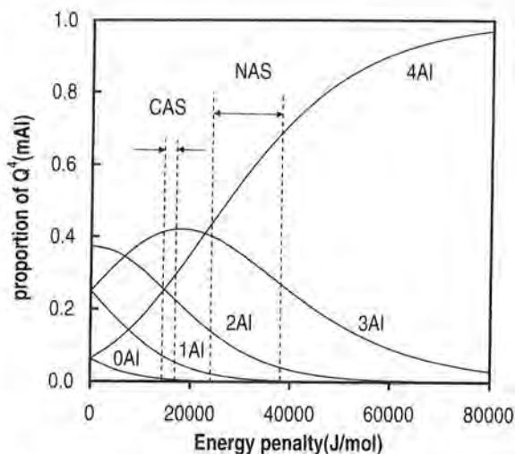
FIGURE 7. Variation of Q^i (mAl) species populations with ordering energy for R=1 . Dashed lines refer the derived degree of Al avoidance ( Q ) for calcium (CAS) and sodium (NAS) aluminosilicate glasses, which range 0.93 \leq Q \leq 0.99 and 0.8 \leq Q \leq 0.875 , respectively. Negative energy penalty is bond ordering enthalpy of Equation 1.
