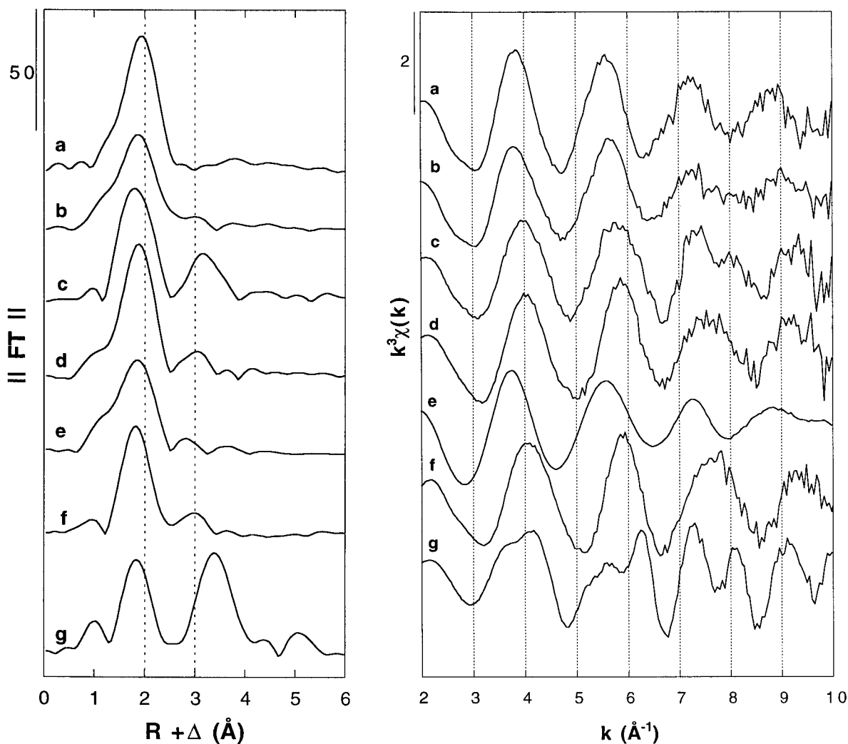
FIGURE 3. Pb L_{III} -EXAFS k^3\chi(k) functions (right) and RDFs (left) of (a) wooded topsoil fine fraction, (b) \text{CaCl}_2 treated wooded topsoil fine fraction, (c) tilled topsoil fine fraction, (d) \text{Na}_4\text{P}_2\text{O}_7 treated tilled topsoil fine fraction, (e) synthetic \text{Pb}^{2+} humate, (f) \text{Pb}^{2+} adsorbed on synthetic goethite, and (g) \text{Pb}^{2+} adsorbed on synthetic birnessite.
