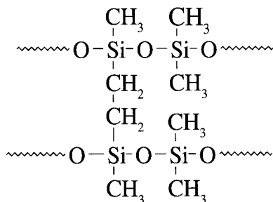
Cross-linked Polydimethylsiloxane
