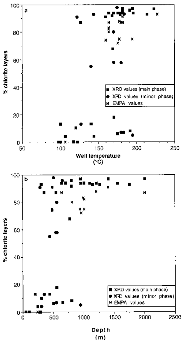
FIGURE 9. Diagram showing percentage chlorite layers as determined by XRD in mafic phyllosilicates in all three wells plotted against (a) well temperature and (b) well depth. The data shows the clear and sharp distinction between smectite with <20% chlorite layers and chlorite with less than ~10% smectite layers.
