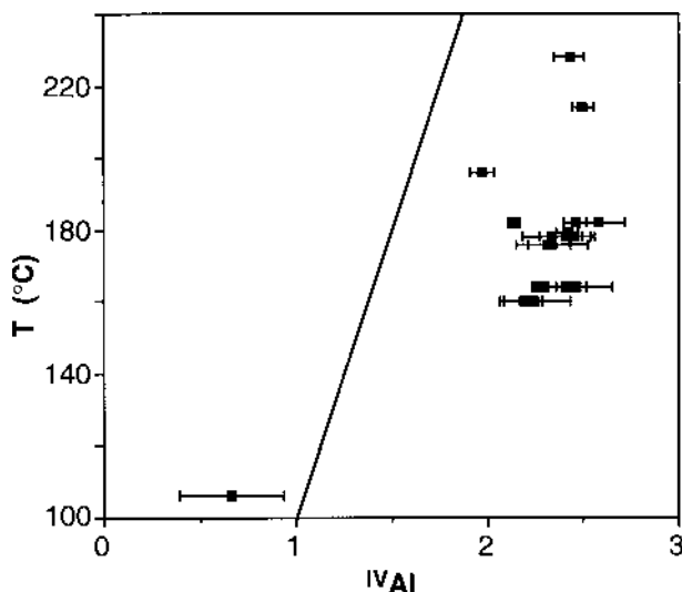
FIGURE 10. Plot of well temperature vs. ^{IV}Al content of mafic phyllosilicates. The Al content is calculated on the basis of variable number of O atoms related to percentage chlorite layers (x), ranging from 22 for a pure smectite to 28 for a clinocllore (Table 1). Straight line shows the relationship derived for the correlation between well temperature and tetrahedral Al content in chlorite from the Azufres geothermal system in Mexico (Cathelineau 1988).
