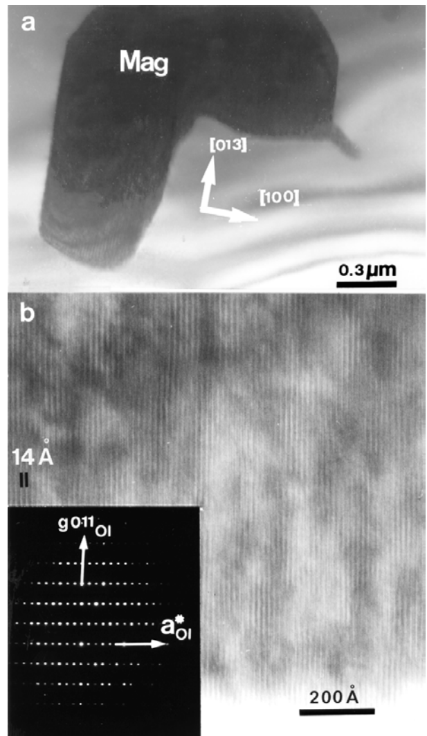
FIGURE 4. (a) Image of a large magnetite particle. (b) The high-resolution image shows fringes with spacing = 14.3\ \text{\AA} . The SAED pattern (inset) of the [011] zone axis of the olivine, also shows the 14.3\ \text{\AA} spacing ( = 3d_{(111)} of magnetite).
