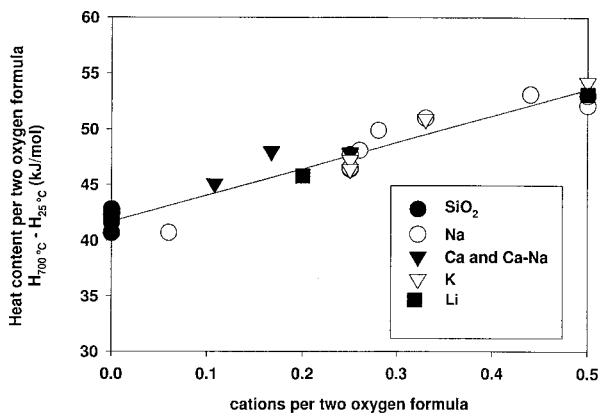
APPENDIX 2—FIGURE 1. Heat content, ( H_{700\text{ }^{\circ}\text{C}} - H_{25\text{ }^{\circ}\text{C}} ) in kJ per two oxygen formula unit as a function of cation content x , in M_x(\text{Si}_y\text{Al}_z)\text{O}_2 framework silicates. Data include dehydrated zeolites, glasses, and dense framework materials. Line is least-squares fit. Data include cristobalite and \text{SiO}_2 glass (Robie and Hemingway 1995), \text{SiO}_2 zeolites (Petrovic et al. 1993); high- and low-albite and \text{NaAlSi}_3\text{O}_8 glass (Robie and Hemingway 1995), nepheline and \text{NaAlSiO}_4 glass (Robie and Hemingway 1995), microcline, sanidine, and \text{KAlSi}_3\text{O}_8 glass (Robie and Hemingway 1995), kaliophillite, leucite, b-eucryptite, and petalite (Robie and Hemingway 1995), dehydrated leonhardite (Kiseleva et al. 1996a), dehydrated analcime (Robie and Hemingway 1995), several Na-faujasites of various Si/Al ratios (Petrovic and Navrotsky 1997), and dehydrated mordenite (Johnson et al. 1992).
