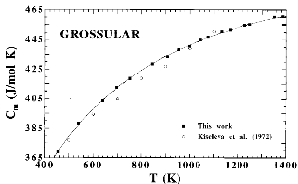
FIGURE 1. Mean heat capacity of grossular. Experimental H_T - H_{273} data of Kiseleva et al. (1972, open circles; referred with Eq. 3 to 273.15 K) and this work (solid squares), and fitted values as given by Equation 3 and the data of Table 4 (solid curve).
