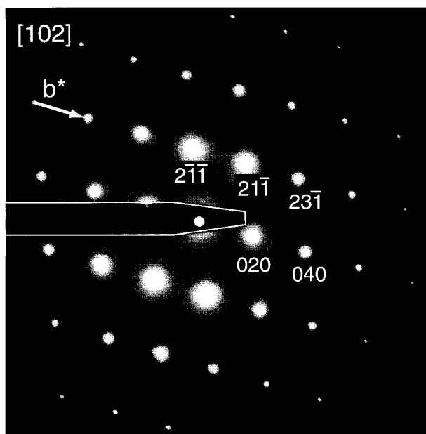
FIGURE 3. Electron diffraction pattern of CaAlFSiO 4 viewed along [102], showing the absence of k + l = 2n + l reflections belonging to space group P2_1/a .
