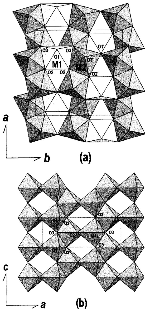
FIGURE 3. The karoosite structure: (a) viewed along c , showing the bands of the M1 and M2 octahedra, and (b) viewed along b , showing the edge-shared M2 octahedral layer. Note the zigzag chains running parallel to the c axis.
