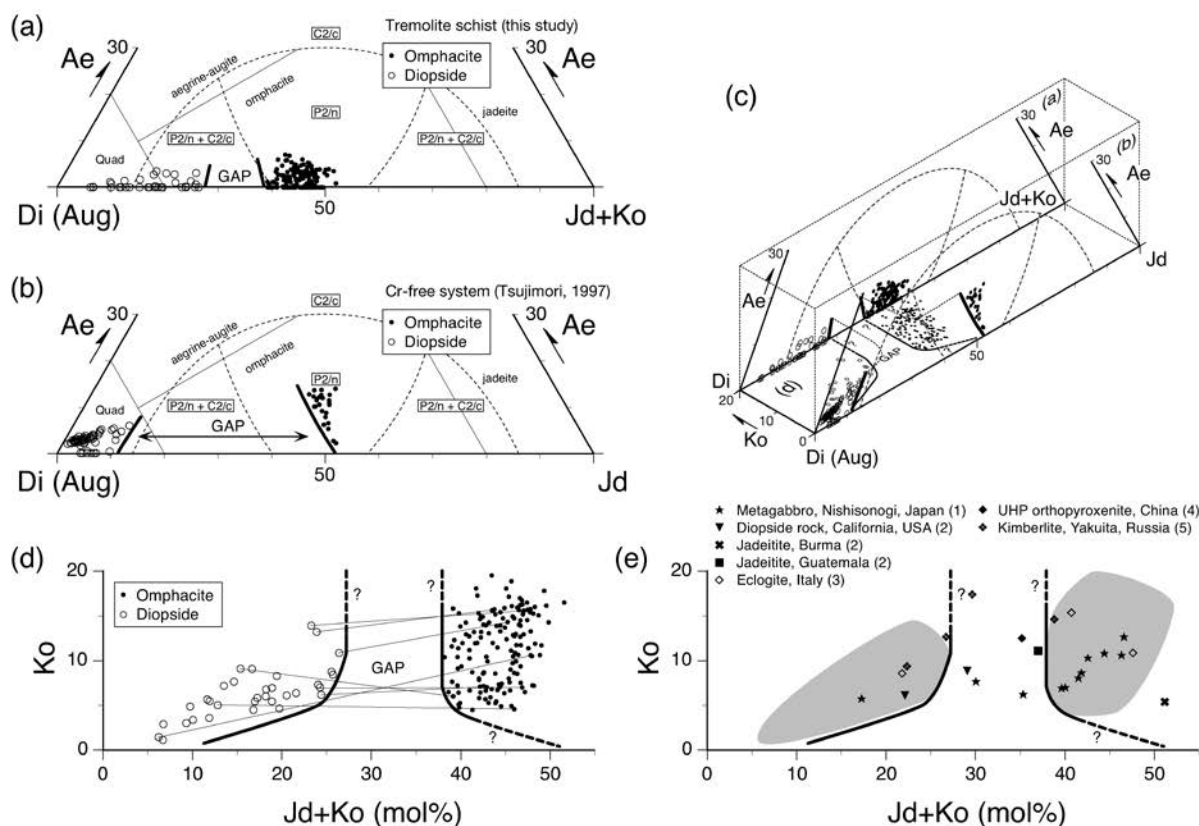
FIGURE 6. Compositional plots of analyzed omphacite and diopside showing the effect of the Ko component on the immiscibility between omphacite and diopside. (a) Compositions of two Cr-bearing clinopyroxenes on the (Jd + Ko)-Di-Ae ternary diagram. The apparent compositional gap is shown as bold lines. Phase relations in the Jd-Di-Ae system proposed by Carpenter (1980b) are also shown as dashed lines. (b) Compositions of coexisting Cr-free omphacite and diopside (augite) from the same outcrop by Tsujimori (1997; additional data) on the Jd-Di-Ae diagram. The compositional gap is shown as bold lines. (c) The three-dimensional illustration showing tentative phase relation between Cr-bearing and Cr-free systems at the same P - T condition. (d) Compositions of two Cr-bearing clinopyroxenes (the present study) on the Ko-(Jd + Ko) diagram. (e) Compositions of the other Cr-bearing omphacitic pyroxenes in literatures (1 = Nishiyama et al. 1986; 2 = Harlow and Olds 1987; 3 = Philippot and Kienast 1989; 4 = Liu et al. 1998; 5 = Sobolev et al. 1975). Hatched areas mean the compositional field of two Cr-bearing pyroxenes plotted in d.
