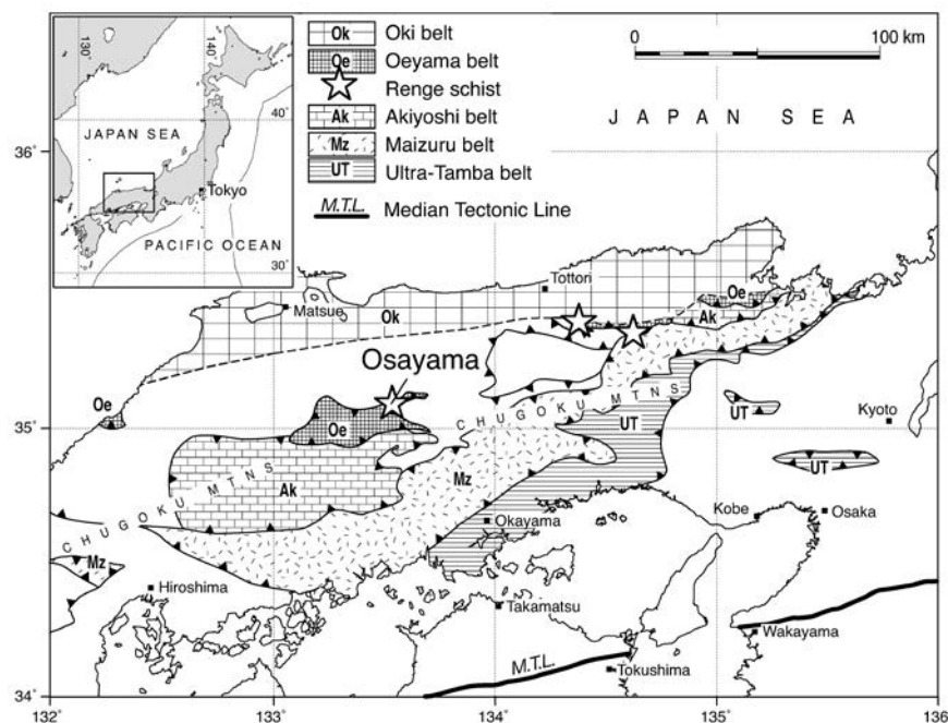
FIGURE 1. Simplified map of the Chugoku Mountains, showing various petroterrestrial units and the sampling locality in the Osayama Mountain (modified after Tsujimori 2002).
