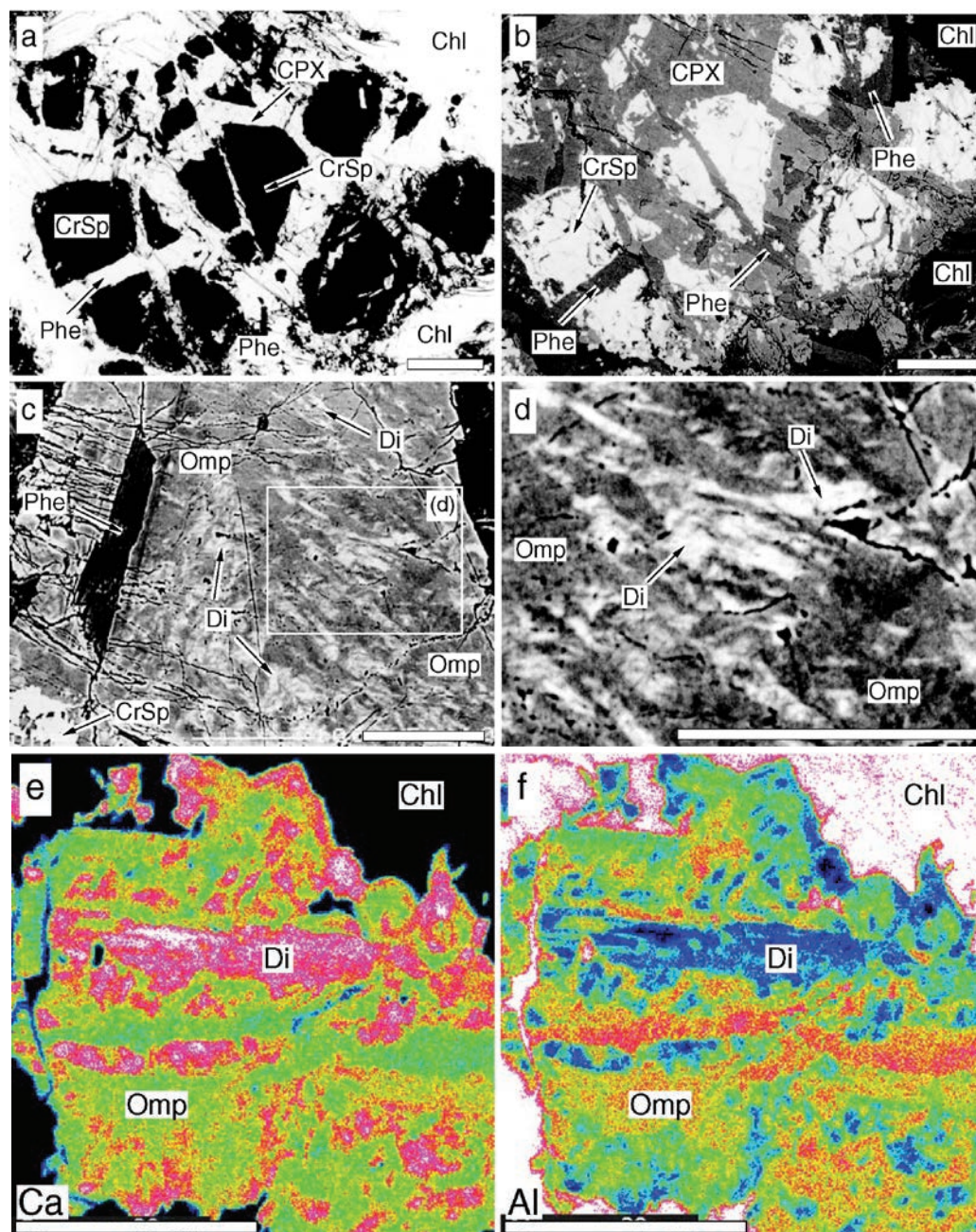
FIGURE 2. Photomicrograph showing occurrences and microtextures of chromian clinopyroxenes in the investigated tremolite schist. (a) Cross-polarized view showing chromian clinopyroxenes (CPX) replacing relict chromian spinel; Cr-bearing matrix minerals including chlorite and phengite are also shown. (b) Back-scattered electron image of same clinopyroxene grain of a. (c) Back-scattered electron image showing lamellae of chromian diopside in chromian omphacite. (d) Enlarged image of a part of chromian diopside lamellae in chromian omphacite. (e) X-ray image of CaK \alpha of coexisting chromian omphacite and diopside. (f) X-ray image of AlK \alpha of e. Scale bars on each image represent 100 \mu m.
