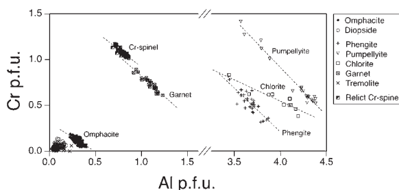
FIGURE 5. Cr vs. Al diagram showing the Cr ↔ Al substitution of analyzed Cr-bearing minerals. The amounts of Cr and Al for these phases are calculated based on their appropriate structural formulae.
