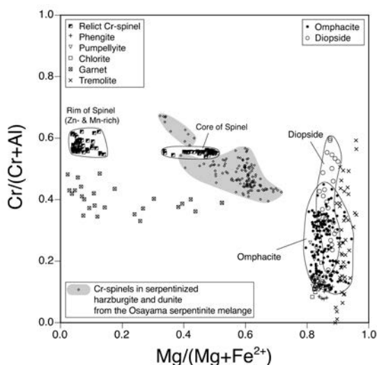
FIGURE 3. Cr/(Cr + Al) vs. Mg/(Mg + Fe 2+ ) diagram showing overall compositional features of analyzed mafic minerals in the tremolite schists. Relict chromian spinels in serpentinized harzburgite and dunite from the Osayama serpentinite melange are also plotted.
