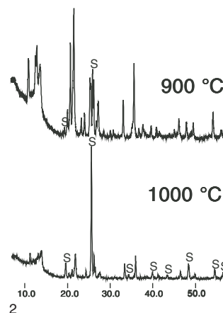
FIGURE 2. Powder XRD patterns of bikitaite at 900 and 1000^\circ\text{C} (experiment C). The peaks labeled S belong to the new phase \gamma -spodumene.
