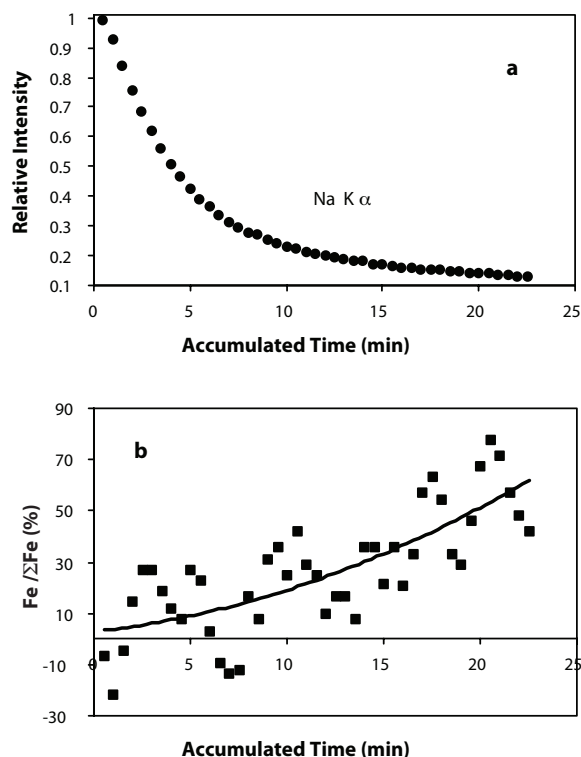
FIGURE 5. (a) Time-dependent loss of the NaK \alpha intensity (measured with a TAP monochromator) within 20–25 min irradiation time for a reduced basaltic glass [with major-element composition (in wt%): MgO=8.1, SiO 2 =50.9, TiO 2 =1.3, Al 2 O 3 =17.5, CaO=10.2, FeO i =6.7, Na 2 O=3.9]. 30s counting time per plot. Same beam conditions as Figure 4. (b) Beam-induced oxidation mechanism of the surface layer of the glass leading \text{Fe}^{3+}/\Sigma\text{Fe} to increase from 6 to 60%. Plots represents 45 successive peak searches (30 s per peak search) performed on a single surface site. The scattering observed for the plots is representative of the average of four replicate series acquired at four different surface sites. No incubation period is apparent for the NaK \alpha intensity loss kinetics indicating rapid migration of Na for this glass composition under the selected beam conditions. In contrast, the oxidation mechanism, involving electron transfer from \text{Fe}^{2+} cations to O atoms left in excess by the removal of Na + , is obviously slower.
