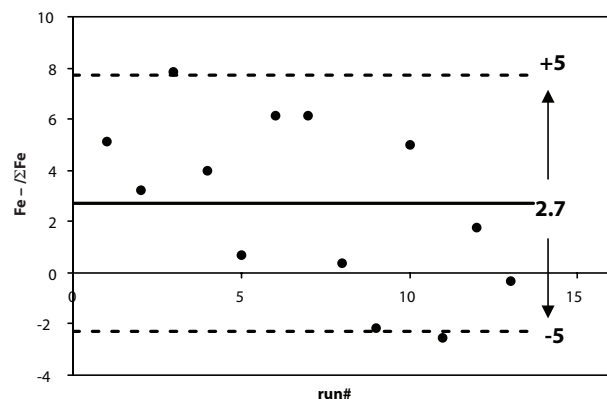
FIGURE 3. \text{Fe}^{3+}/\Sigma\text{Fe} measured from a San Carlos olivine with 7.4 wt% Fe. Operating conditions: 15 keV, 240 nA, 20 \mu\text{m} , 60 peak searches integrated per plot (30 min acquisition). This result, namely \text{Fe}^{3+}/\Sigma\text{Fe} = 2.7 \pm 5\% ( 2\sigma precision), can be taken as a measure of the intrinsic accuracy and precision expected for the series of reference glasses (with Fe concentration ranging from 6 to 9 wt%) of this study.
