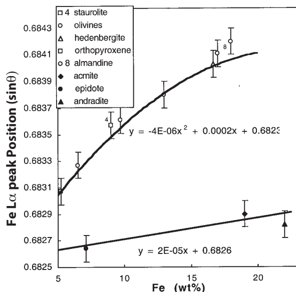
FIGURE 2. Variations of the \text{Fe}L\alpha peak position measured at 15 keV with a TAP monochromator as a function of the total Fe concentration (5–20 wt% Fe) for a series of pure \text{Fe}^{2+} -bearing and pure \text{Fe}^{3+} -bearing silicates (plots are partially reprinted from Fig. 3 in Fialin et al. 2001). Numbers next to symbols in the legend indicate coordination numbers of Fe ions for minerals in which coordination numbers are not six. First- and second-order polynomial fits are shown.
