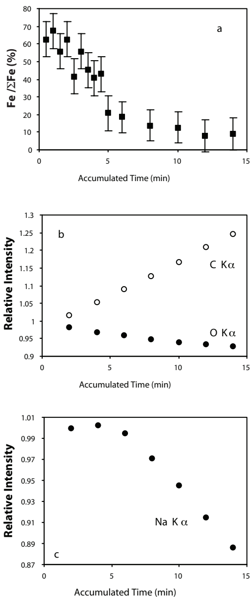
FIGURE 6. (a) Reduction kinetics for a mixed \text{Fe}^{2+} - \text{Fe}^{3+} glass [major-element composition (in wt%): MgO = 9.9, SiO 2 = 52.9, CaO = 16.9, FeO i = 12.6, Na 2 O = 5.9] whose \text{Fe}^{3+}/\Sigma\text{Fe} decreases from 65 to less than 10% within 15 min irradiation time (same beam conditions as Fig. 4 excepted 30 \mu\text{m} spot diameter). Plots above (resp. below) 5 min result from peak searches of 2 min (resp. 30s), and they are the average of three (resp. ten) replicate measurements at three (ten) fresh surface sites. (b) Time-dependent evolution of the OK \alpha intensity (measured with a W/Si metallic multilayer monochromator, or MMM, with 2d = 6\text{nm} ) and the CK \alpha intensity (measured with a Ni/C MMM with 2d = 9.5\text{nm} ). These plots show that the reduction of the surface layer is not related to the removal of oxygen atoms. The loss of OK \alpha intensity is correlated with the carbon contamination build-up due to cracking of pump oil molecules present in the sample chamber. 2 min counting time per plot. (c) Time-dependent loss of NaK \alpha intensity showing that the reduction mechanism occurs during the incubation period of Na.
