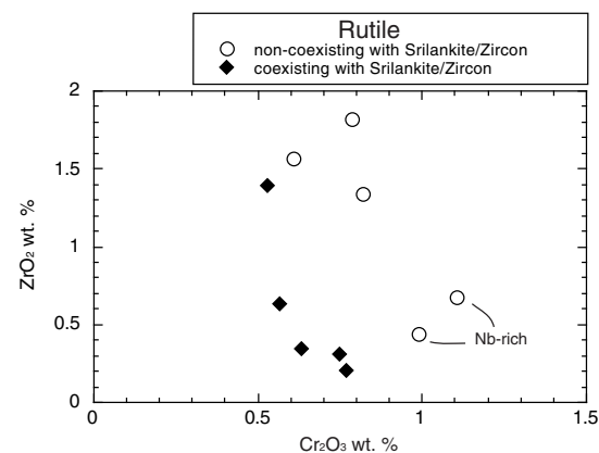
FIGURE 6. wt% Cr_2O_3 vs. wt% ZrO_2 of rutile in the gabbroic vein.
