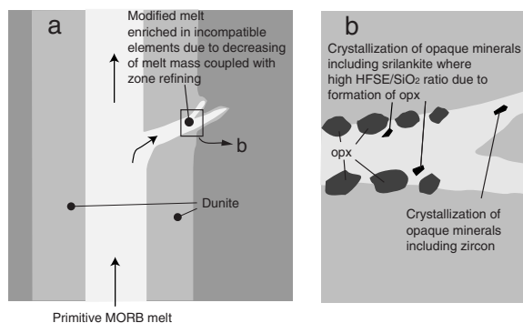
FIGURE 7. Schematic model showing the melt-mantle interactions. (a) The formation of a modified melt due to interaction between ilmenite and a primary MORB melt resulting in the formation of dunite as a melt conduit. The modified melt was enriched in incompatible elements due to decreasing of melt mass coupled with a zone-refining effect. See text for more details. (b) The precipitation of srilankite from the modified melt. Srilankite might be formed locally in high HFSE/SiO 2 areas where orthopyroxenes (opx) were formed by interaction with host peridotite and the modified melt.
