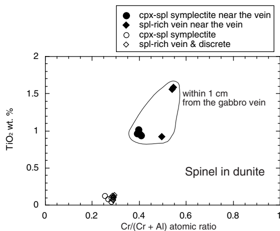
FIGURE 4. The \text{Cr}' [= \text{Cr}/(\text{Cr} + \text{Al}) atomic ratio] vs. wt% \text{TiO}_2 of spinels in the dunite host. Spl-rich vein = spinel in spinel-rich vein in the studied sample.
