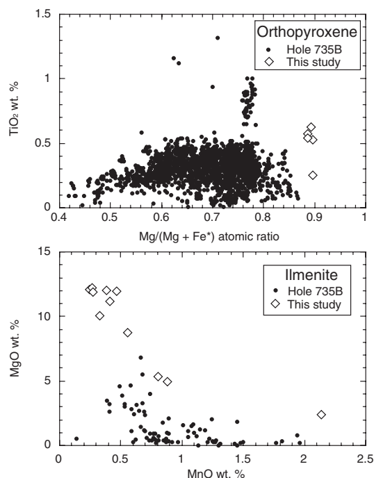
FIGURE 5. Comparisons of mineral compositions from the gabbroic vein and the gabbros from Hole 735B. (a) Mg' [=Mg/(Mg + Fe*)] atomic ratio: Fe* = total iron as Fe] vs. wt% TiO_2 of orthopyroxene. Orthopyroxene compositions in the gabbros of Hole 735B are from Dick et al. (2002). (b) wt% MgO vs. wt% MnO of ilmenite. Ilmenite compositions in the gabbros of Hole 735B are from Natland et al. (1991), Hébert et al. (1991), Hertogen et al. (2002), and Niu et al. (2002).
