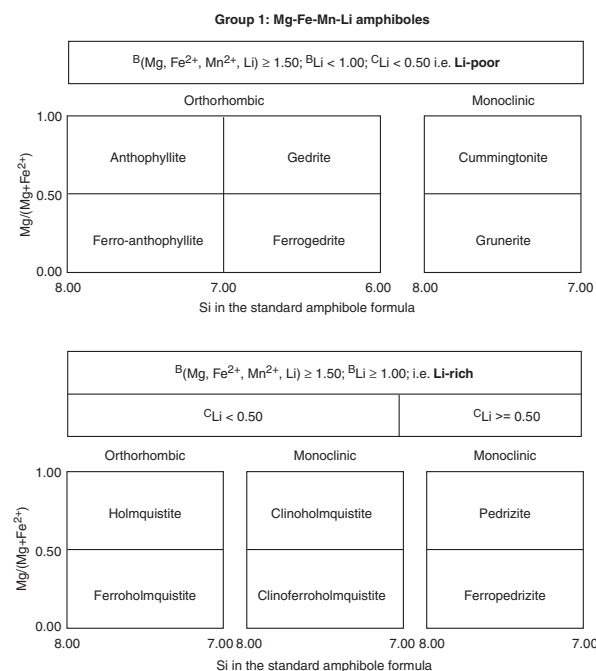
FIGURE 1. Classification of the Group 1 amphiboles; Mg-Fe-Mn-Li amphiboles.
