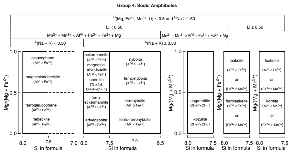
FIGURE 2. Classification of the Group 4 amphiboles; sodic amphiboles.
