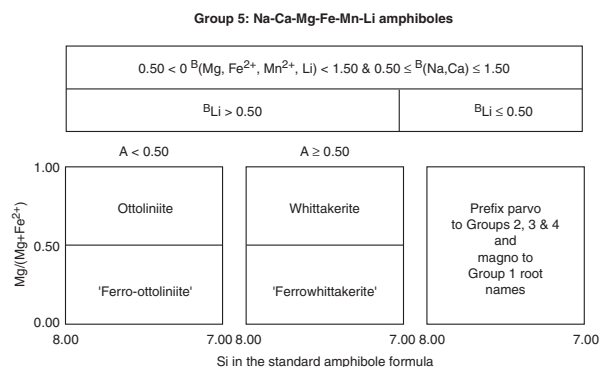
FIGURE 3. Classification of the Group 5 amphiboles; Na-Ca-Mg-Fe-Mn-Li amphiboles.
