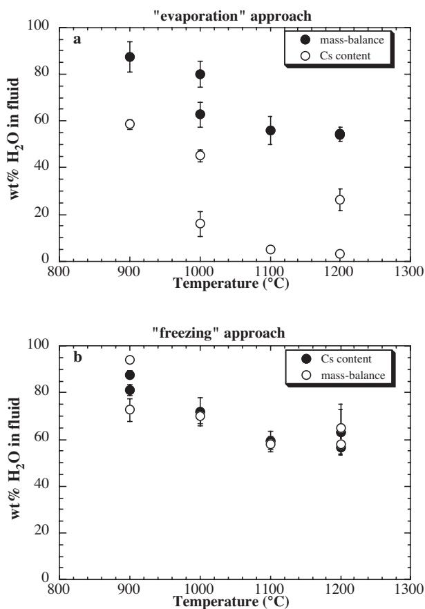
FIGURE 6. (a) The \text{H}_2\text{O} concentrations (wt%) of fluids in capsules treated following the “evaporation” approach obtained from mass balance compared to those calculated using the Cs signal. (b) The \text{H}_2\text{O} concentrations (wt%) of fluids in capsules treated following the “freezing” approach obtained by using the Cs signal compared to those based on mass balance calculations. Each symbol represents an average and one standard deviation of the distribution of analyses.
