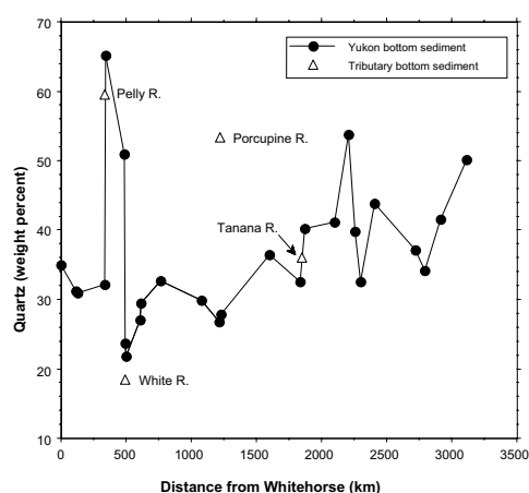
FIGURE 5. Wt% quartz in bed sediments with distance from Whitehorse.
