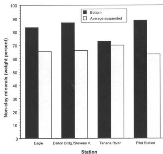
FIGURE 15. A comparison between wt% non-clays in bed and suspended sediments for four fixed stations. The values for the suspended sediments are average values for the 2002 season.
