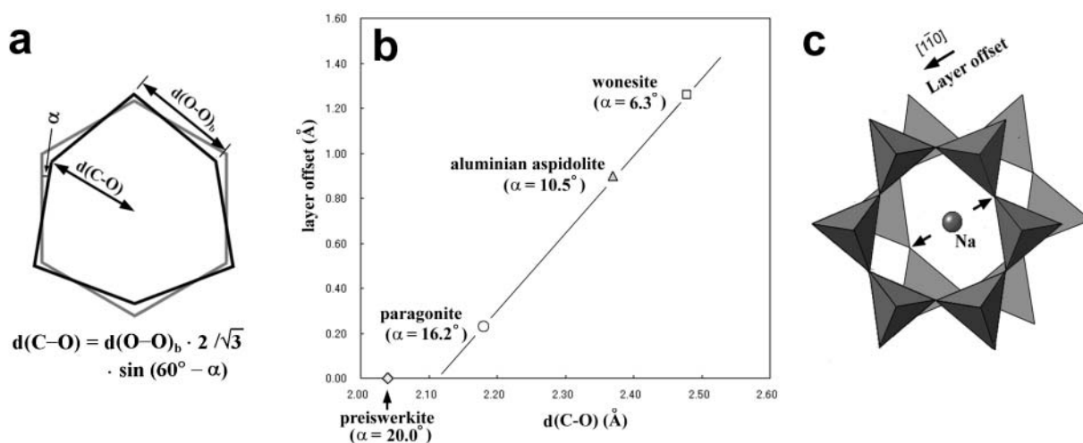
FIGURE 7. (a) Definition of d (C-O), the distance between the center of the oxygen hexagonal ring and the closest oxygen atoms, and the equation to calculate d (C-O) from the averaged neighboring O-O distance [ d (O-O) b ] and ditrigonal rotation angle (α). (b) The relationship between d (C-O) and the layer offset in four sodium micas. α's for aspidolite and wonesite were calculated from the composition for the 2:1 layer using the formula by Weiss et al. (1992). (c) Schematic illustration to show the layer offset between two tetrahedral hexagonal rings across the interlayer region in wonesite. The sodium atom is assumed to be located at the center of the staggered cavity space.
