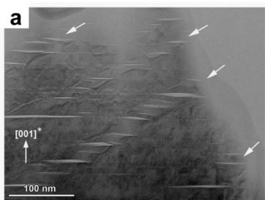
FIGURE 6. (a) TEM micrograph to show talc lamellae (indicated with the white arrows) in wonesite. The beam direction is close to one of [010], [310], or [310]. Lens-like voids are observed in the lamellae as reported by Veblen (1983a). (b) Experimental XRD pattern from wonesite and calculated patterns for wonesite (dark line) and for talc (gray line). The two patterns were calculated by assuming the volume ratio of wonesite and talc to be 4:1. The peak profile for the calculation is the same as that in Figure 3. The two squares on the pattern indicate the areas magnified in c and d . (c, d) Portions of the figure in b to show the distinct peaks of talc in the experimental pattern. (e) Experimental XRD patterns around 003 of wonesite from five different grains. The center, right, and left peaks are 003 of wonesite, talc, and phlogopite, respectively. Note that the intensity ratio between the peaks of wonesite and talc is comparable between the five patterns.
