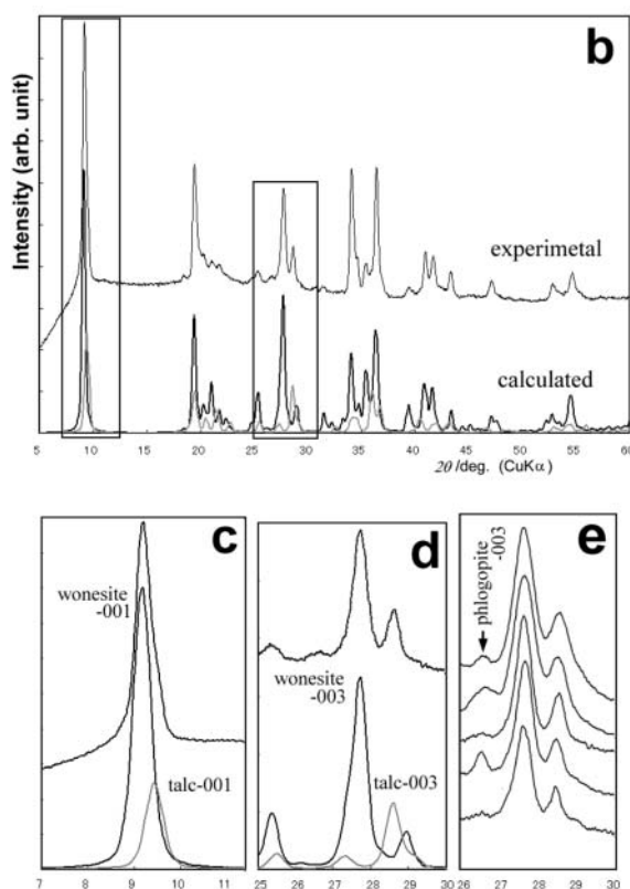
FIGURE 6. (a) TEM micrograph to show talc lamellae (indicated with the white arrows) in wonesite. The beam direction is close to one of [010], [310], or [310]. Lens-like voids are observed in the lamellae as reported by Veblen (1983a). (b) Experimental XRD pattern from wonesite and calculated patterns for wonesite (dark line) and for talc (gray line). The two patterns were calculated by assuming the volume ratio of wonesite and talc to be 4:1. The peak profile for the calculation is the same as that in Figure 3. The two squares on the pattern indicate the areas magnified in c and d . (c, d) Portions of the figure in b to show the distinct peaks of talc in the experimental pattern. (e) Experimental XRD patterns around 003 of wonesite from five different grains. The center, right, and left peaks are 003 of wonesite, talc, and phlogopite, respectively. Note that the intensity ratio between the peaks of wonesite and talc is comparable between the five patterns.
