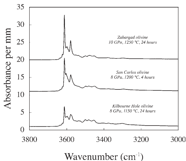
FIGURE 4. Synthetic E lla IR spectra for olivine from three different experiments that used three different starting materials. The starting olivine material and conditions of the experiments are annotated in the figure. The run numbers (see Table 1), starting from the top of the figure going down, are ww256, ww325, and ww227.
