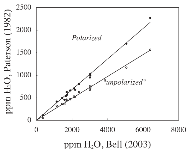
FIGURE 8. Comparison among IR calibrations applied to our experimental samples. Filled and unfilled circles are for polarized and unpolarized IR spectra, respectively. Spectra were calculated as discussed in the text. Regression lines constrained to pass through the origin indicate that the Bell et al. (2003) calibration gives 2.95 or 4.12 times the amount of the Paterson (1982) calibration for polarized and unpolarized radiation, respectively.
