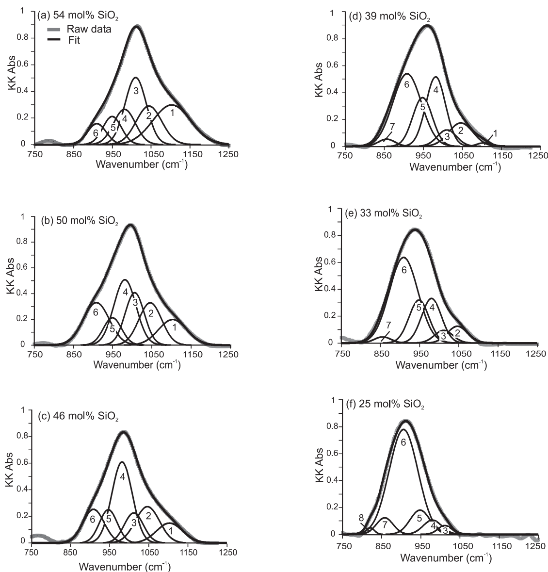
FIGURE 5. The deconvoluted bands from Fit 1 (from high to low wavenumber), obtained for the (a) 54 mol% \text{SiO}_2 glass; (b) 50 mol% \text{SiO}_2 glass; (c) 46 mol% \text{SiO}_2 glass; (d) 39 mol% \text{SiO}_2 glass; (e) 33 mol% \text{SiO}_2 glass; and (f) 25 mol% \text{SiO}_2 glass. A total of eight bands were used, at center values ( \text{cm}^{-1} ) within 5% of those predicted from the 2nd derivative of the \mu\text{R-FTIR} spectra.
