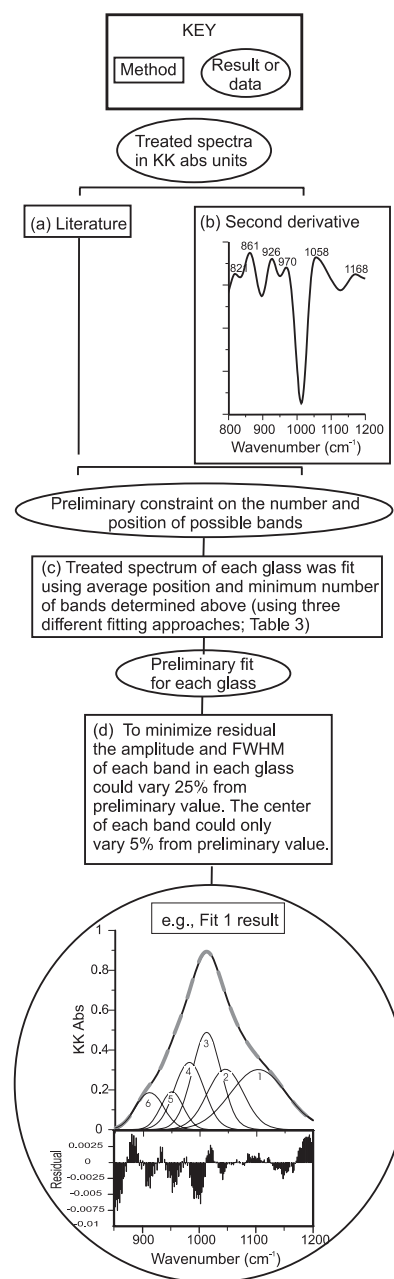
FIGURE 2. Flow chart illustrating the steps taken to deconvolve Voigt-shaped bands from the treated spectra (in all three fitting methods). First, a literature search on the position of Raman and IR bands of silicate glasses (a), and the calculation of the second derivative of the spectra (b), provided a preliminary constraint on potential band characteristics. The treated spectra were fit with bands at centers close to those predicted from methods a and b (using three different fitting approaches) to produce preliminary fits (c). During the final iteration process (d), both the amplitude and FWHM of each band was free to vary with 25% of the amplitude determined in the preliminary fits and the center of each Voigt-shaped band was constrained to within 5% of the center determined in the preliminary fits. The goodness of the resultant fits (Fit 1 illustrated) is monitored using a plot of the residuals, where there was <0.02 KK abs difference between the real and reconstructed spectra.
