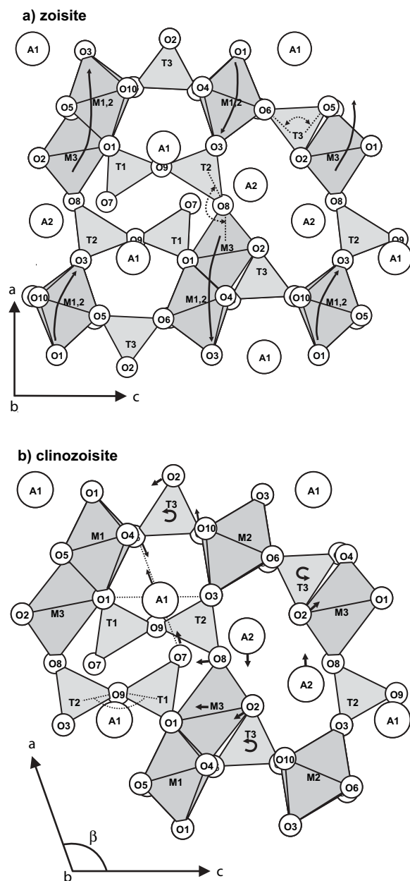
FIGURE 11. (a) Displacement of the octahedron blocks in zoisite in response to Sr incorporation; displacement is shown with bold arrows. Laterally linked T3 turn and T1-T2 group is bended by this displacement (dotted arrows). (b) Decrease in angle \beta in clinozoisite, compression of M3 and T3 polyhedra and elongation of the A1-O6 distance in response to Sr-incorporation. Rotation of T3 with O5 toward A1 is combined with a volume decrease in T1 at X_{Sr} \approx 0.25 , O7-A1 distance relax after that movement (see text).
