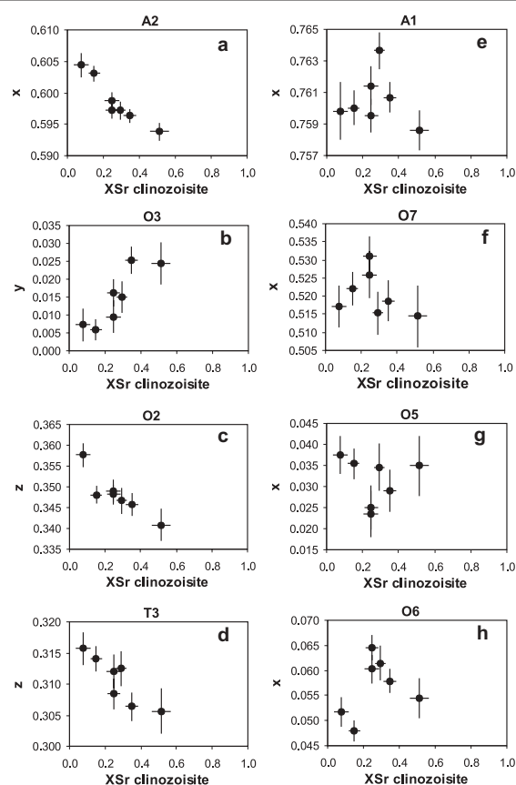
FIGURE 7. (a–h) Changes in atomic positions for atoms A1, A2, O2, O3, O5, O6, O7, and T3 in clinozoisite with increasing X_{Sr} .
