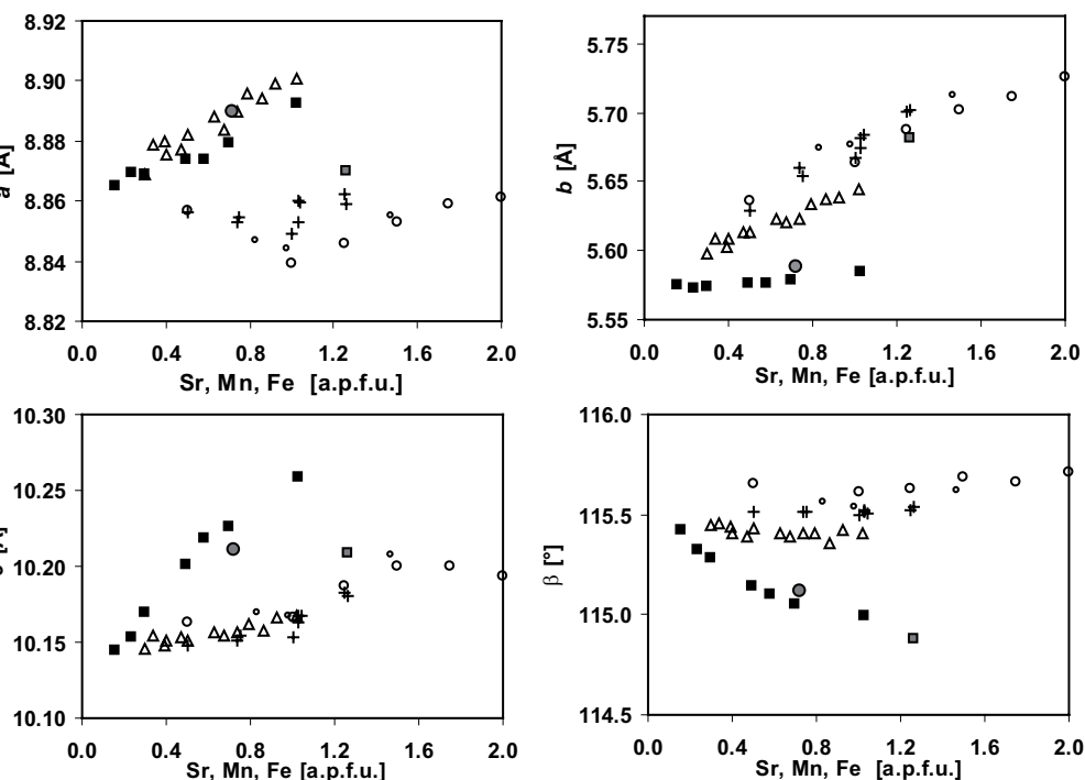
► FIGURE 10. Comparison of the variation in lattice parameters due to the Ca-Sr-substitution on A1 and A2 in clinozoisite (filled squares, this work), compared with Al-Fe-substitution in clinozoisite (open triangles, Carbonin and Molin 1980; Bonazzi and Menchetti 1995) and Al-Mn-substitution in piemontite (open circles, Anastasiou and Langer 1977; small open circles, Langer et al. 2002; cross, Nagashima et al. 2004) on the M-sites. Data points for niigataite (gray circle, Miyajima et al. 2003) and strontioziemontite (gray square, Bonazzi et al. 1990) lie between the series.
