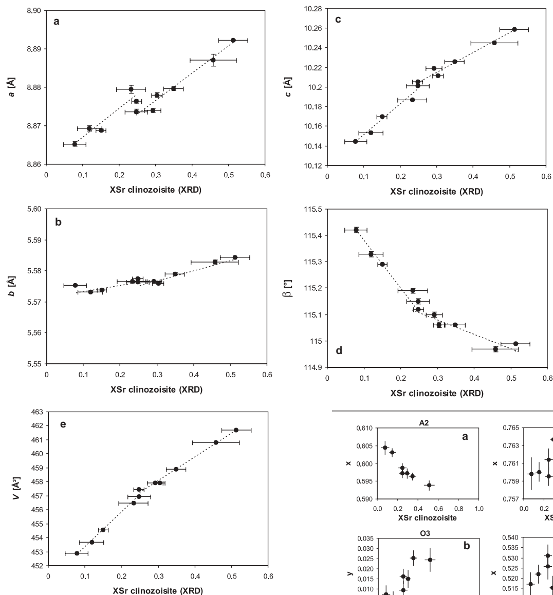
FIGURE 6. (a–e) Variation of Ca-Sr clinozoisite lattice parameters with X_{Sr} in the range X_{Sr} = 0.08 to X_{Sr} = 0.5 . Lattice parameter b does not change significantly, whereas the angle \beta decreases. A discontinuity at X_{Sr} \approx 0.25 is most visible in lattice parameter a and angle \beta . Dotted lines are visual fits.
