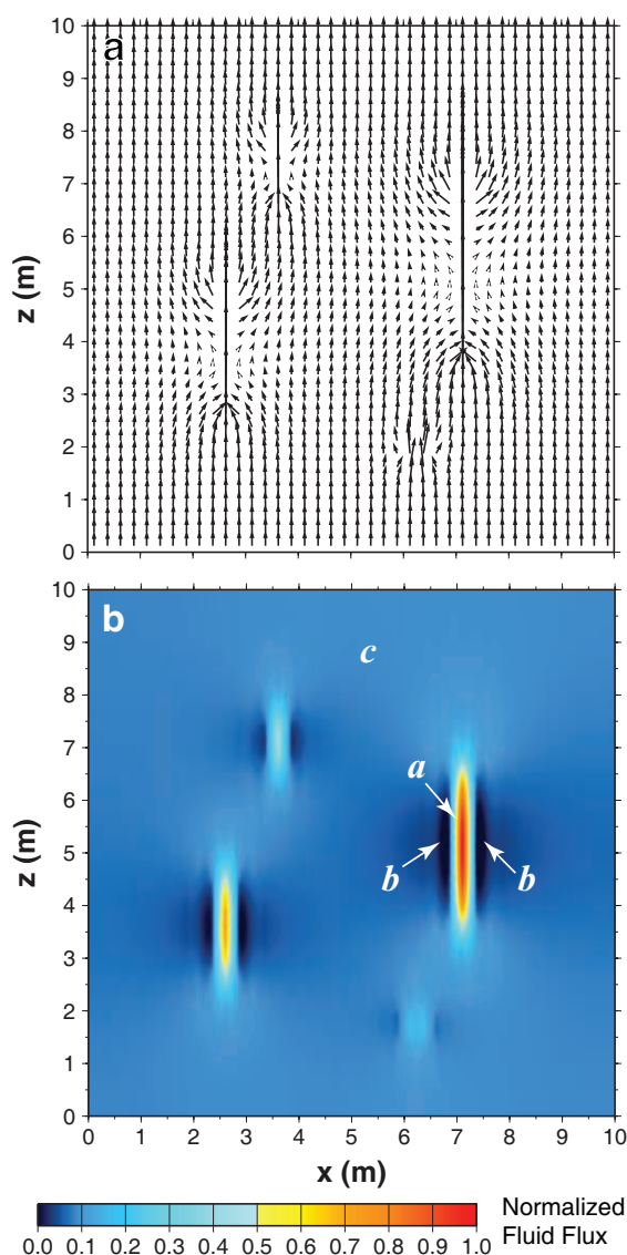
FIGURE 11. Simple two-dimensional models of upward fluid flow. (a) Vectors illustrating magnitude and direction of fluid flow; vector length scales with flux magnitude. Note focusing of flow into four high permeability zones (model fractures) of varying lengths. (b) Fluid fluxes normalized to the maximum flux value. Largest fluxes are predicted in the model fractures and directly at fracture-rock contacts (e.g., point a ). Channelization of fluid into the fractures impoverishes the surroundings in fluid such that the lowest flux areas are found adjacent to the fractures (e.g., points labeled b ). “Background” fluxes away from fractures are also small (e.g., point c ).
