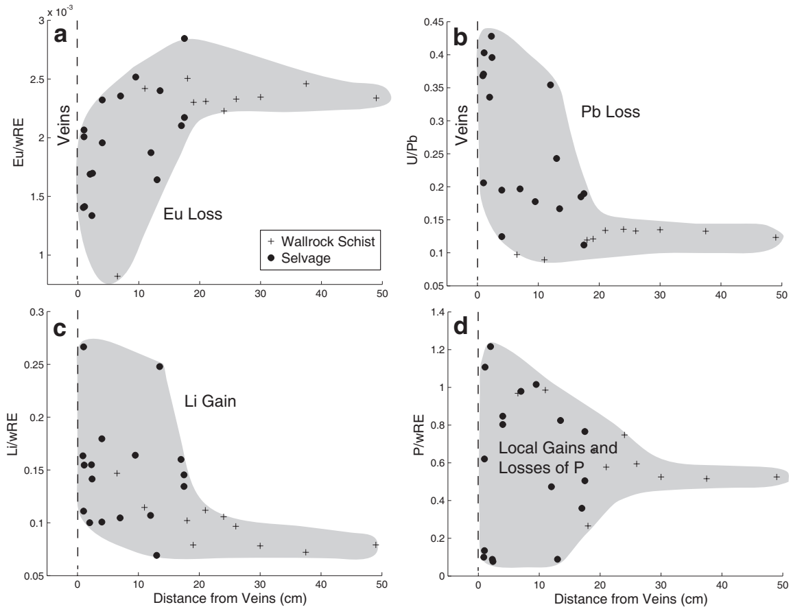
FIGURE 9. Geochemical profiles. Data for all three traverses plotted on the same x-axis. (a) \text{Eu}/w\text{RE} . Decrease in Eu concentration relative to w\text{RE} reference frame indicates mass loss. (b) \text{U}/\text{Pb} . U was essentially immobile but Pb was lost, resulting in increases in \text{U}/\text{Pb} toward veins. (c) \text{Li}/w\text{RE} . (d) \text{P}/w\text{RE} .
