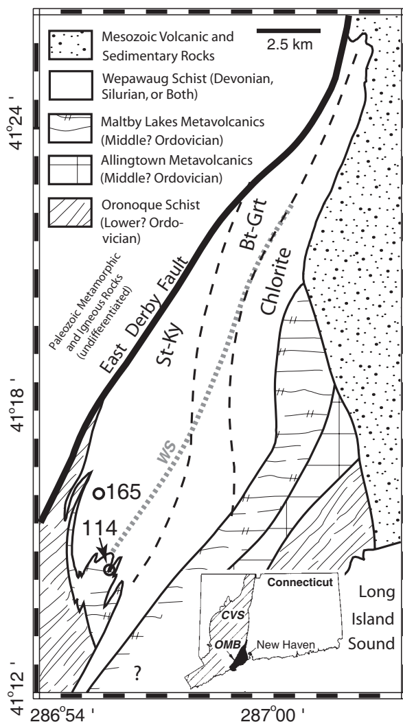
FIGURE 1. Geologic sketch map of the Wepawaug Schist, part of the Orange-Milford belt (OMB) of the Connecticut Valley Synclinorium (CVS). Sample localities JAW114 and JAW165 shown with open circles (prefix JAW omitted for clarity). WS = Axis of Wepawaug syncline. Modified after Fritts (1963, 1965a, 1965b) and Rodgers (1985). Isograd positions after Ague (2003a).
