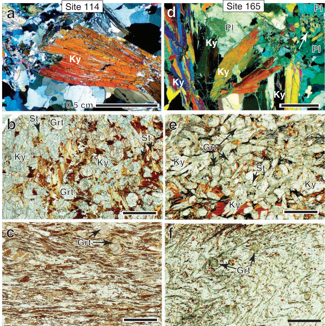
FIGURE 3. Photomicrographs. Parts (a) and (d) under crossed polars; remainder under plane-polarized light. Scale bars = 0.5 cm. Parts (a–c) Vein-selvage relations, site 114. (a) Large kyanite (Ky) blades in quartz vein. (b) Kyanite- and garnet-rich (Grt) selvage. Staurolite (St) and biotite (dark) also present. Abundant dark “specks” in the photo are mostly rutile and zircon crystals, concentrated due to silica loss. (c) Wallrock schist distal to veins rich in quartz and plagioclase (light) and bands of muscovite + biotite. Parts (d–f) Vein-selvage relations, site 165. (d) Kyanite blades cutting slightly sericitized, pre-existing plagioclase (Pl) in vein. Arrow denotes plagioclase almost completely replaced by small kyanite crystals (light). (e) Kyanite- and garnet-rich selvage. Biotite (dark) also present. Concentrations of organic matter in bands and between grains appear black. (f) Wallrock schist distal to vein is dominated by contorted quartzofeldspathic (light) and muscovite+biotite bands.
