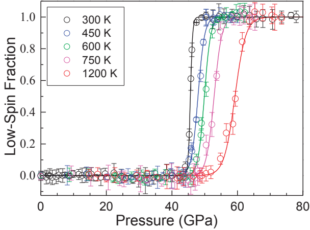
FIGURE 4. Low-spin fraction of magnesiosiderite [(\text{Mg}_{0.35}\text{Fe}_{0.65})\text{CO}_3] as a function of pressure compared with the fitting results. Open circles: experimental measurements; lines: fitting results. Vertical ticks represent the error for the low-spin fraction. Errors are calculated using standard error propagations from our modeled parameters. (Online color.)
