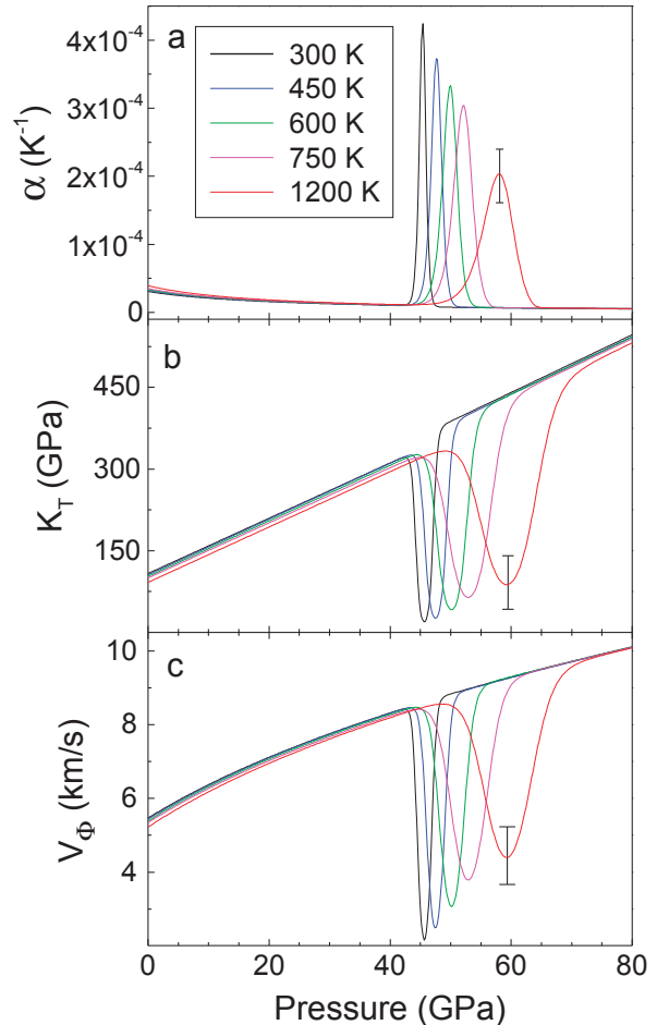
FIGURE 6. Thermal elastic parameters of magnesiosiderite [(\text{Mg}_{0.35}\text{Fe}_{0.65})\text{CO}_3] at constant temperatures. \alpha = thermal expansion coefficient; K_T = isothermal bulk modulus; V_\Phi = bulk sound velocity. Vertical ticks = representative errors ( \pm 1\sigma ) for \alpha , K_T , and V_\Phi , respectively. (Online color.)
