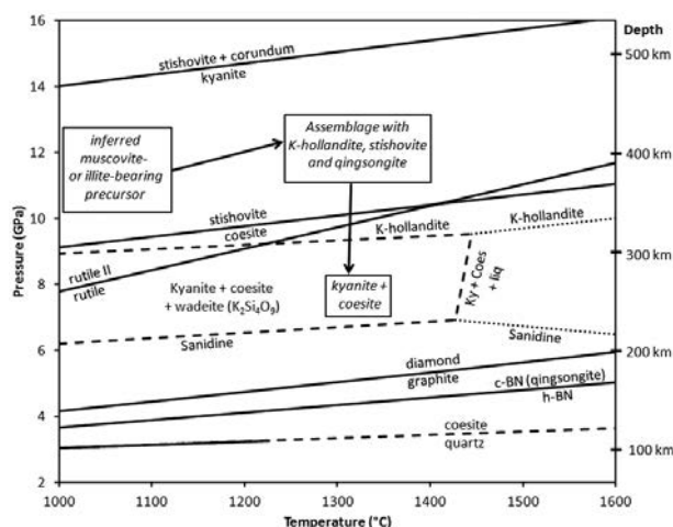
FIGURE 9. Pressure-temperature diagram showing reactions relevant to the formation conditions and origin of qingsongite. Sources of data: hexagonal-BN (h-BN) \leftrightarrow c-BN (Corrigan and Bundy 1975); graphite \leftrightarrow diamond (Day 2012); reactions involving K-bearing phases in the system \text{KAlSi}_3\text{O}_8 , dashed where some experimental constraints and dotted where estimated (simplified from Urakawa et al. 1994); coesite \leftrightarrow stishovite (Akaogi et al. 2011); rutile \leftrightarrow rutile II (Withers et al. 2003); kyanite \leftrightarrow stishovite + corundum (Schmidt et al. 1997); coesite \leftrightarrow quartz, dashed where extrapolated (Hemingway et al. 1998). Boxes and arrows mark the evolution of the qingsongite-bearing fragment.
