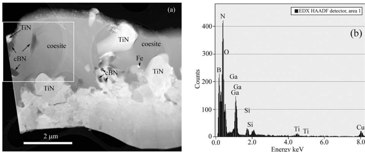
FIGURE 2. (a) A part of the TEM foil exhibits coesite matrix (light gray contrast), osbornite (TiN, bright contrast), qingsongite (c-BN, darker gray contrast) (modified from Dobrzhinetskaya et al. 2009). (b) Energy-dispersive X-ray spectrum shows presence of intense peaks for boron = B and nitrogen = N (inclusion of qingsongite) considering the small fluorescence yields of boron and nitrogen. Ga-peak originates from Ga-implantation during the TEM foil preparation with FIB; Cu X-ray intensity is from the TEM Cu-grid; Si and O X-ray intensities are from matrix coesite; and Ti is from neighboring osbornite.
