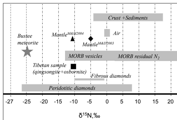
FIGURE 8. Nitrogen isotope characteristics of selected materials. Data source: Bustee meteorite (Carr and Pillinger 1984); Tibetan sample (this study); Crust, Sediments, Air, MORB, and diamonds (Javoy 1997); Mantle M&D2003 (Marty and Duphas 2003) and Mantle M&M2004 (Mohaparta and Murty 2004).
