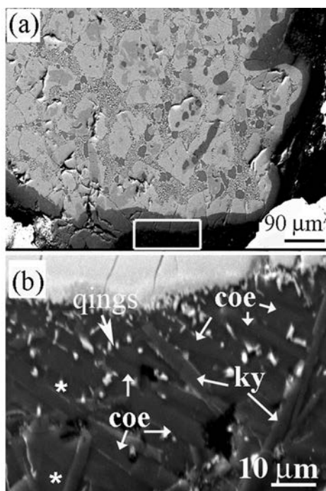
FIGURE 1. Scanning electron microscope images of the rock sample containing qingsongite (from Dobrzhinetskaya et al. 2009). (a) Backscattered electron image of Fe-Ti pellet rimmed by silicate rock (boxed area). (b) Detail of the boxed area shows silicate material containing coesite (coe), kyanite (ky), qings (qingsongite), unknown amorphous phase (*) of the composition: ( \text{SiO}_2 = 63.00 , \text{Al}_2\text{O}_3 = 14.50 , \text{TiO}_2 = 9.02 , \text{CaO} = 0.5 , \text{MgO} = 4.26 , \text{K}_2\text{O} = 5.16 , in wt%), and osbornite (bright spots).
