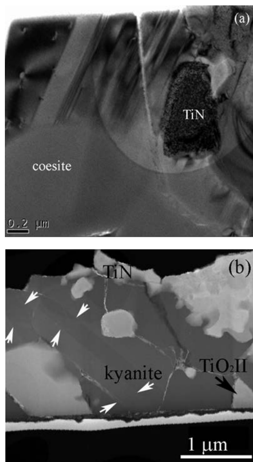
FIGURE 6. TEM images showing: (a) bright-field image of coesite with twin lamellae containing an inclusion of osbornite; (b) HAADF image with twin lamellae in kyanite (white arrows) containing inclusions of osbornite and \text{TiO}_2 II.
