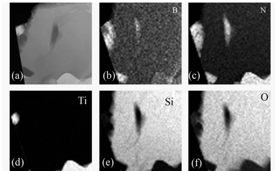
FIGURE 4. EDX element maps of the area boxed on Figure 2. (a) An image of the mapped area, (b) boron, (c) nitrogen, (d) titanium, (e) silicon, and (f) oxygen.
