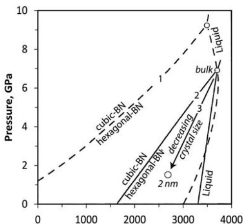
FIGURE 7. Boron nitride phase diagram modified from Solozhenko (1995). The c-BN–h-BN–liquid triple point is marked by a circle. (1) Dashed line based on Bundy and Wentworth (1963) is essentially the same as reported by Corrigan and Bundy (1975). (2) Solid line is based on the “equilibrium diagram” derived by Solozhenko et al. (1990). (3) Arrow labeled in italics indicates decrease in pressure and temperature of the triple point with decrease in crystal size to 2 nm calculated from the thermodynamic theory at the nanoscale by Hu et al. (2011).
