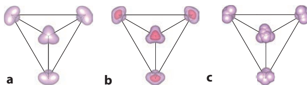
FIGURE 7. Disorder of oxygen ions tetrahedrally surrounding the Li ion in the low- and high-temperature forms of \text{LiMn}_2\text{O}_4 viewed along [111] of the cubic prototype: (a) the atomic displacement parameter (ADP) ellipsoids of 12 oxygen ions with 33.3% occupation around Li, obtained from the harmonic 96g model for the high-temperature form at 320 K; (b) the joint-probability density function (j-pdf) of 4 oxygen ions obtained from the anharmonic (up to the fourth-order) 32e model for the high-temperature form at 320 K, and (c) the statistical distribution of oxygen ions at 230 K in the low-temperature form, superimposed onto a \text{LiO}_4 tetrahedron by translation operation. The ADP ellipsoids in a are drawn at the 95% probability level, and the j-pdf of the oxygen ions in b is drawn using two isosurfaces of 50 and 95% probability levels from inside, and the oxygen ions in c are depicted using spheres of 0.6 Å in radius.
