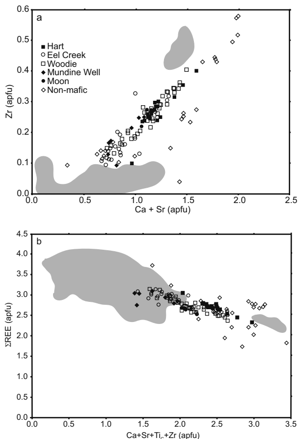
FIGURE 5. Elemental plots for c/p from tholeiitic mafic rocks compared with data from other common rock types (shaded fields and open diamond symbols). Analyses from tholeiites have more Zr than most rock types, but less than Zr-enriched analyses. (a) Ca+Sr vs. Zr (apfu). (b) Ca+Sr+Ti in C-site + Zr vs. total REE. Legend in b as for a.
