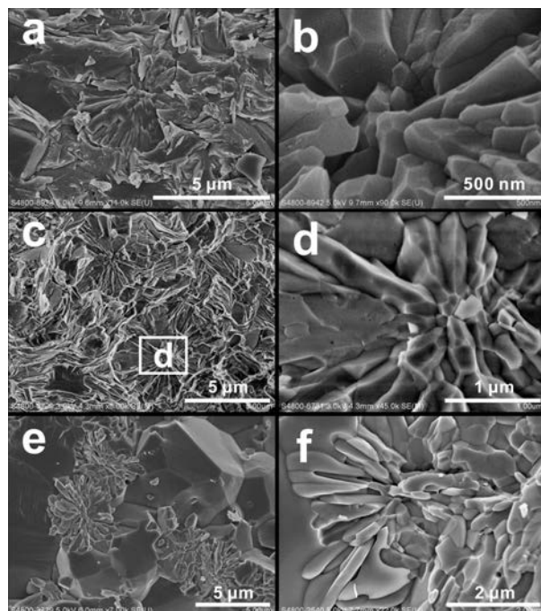
FIGURE 4. SEM images of apatite from Neoarchean to Paleoproterozoic BIFs. (a–b) apatite flowers from the Kuruman BIF, b shows the polyhedral apatite particles in the flower center. (c–d) Apatite flowers from the Dales Gorge BIF, c shows flow structures of the siliceous minerals around the apatite flowers, d shows the magnified image of the apatite grains in the flower center in c. (e–f) Apatite flowers from the Abitibi BIF, quartz in Abitibi BIFs shows polyhedral shapes.
