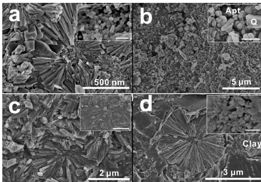
FIGURE 3. SEM images of apatite from Mesoproterozoic to Neoproterozoic sedimentary rocks. (a) Flower-like apatite from Kaiyang phosphorite with petals of straight boundaries and smooth surfaces, inset shows the compacted polyhedral fine-grained apatite crystals in the flower centers. (b) Nanoparticles of apatite from the Yangtze Gorges cherty nodule, inset is a magnified image of the fine-grained apatite coexisting with euhedral quartz. (c) Flower-like apatite from Yangtze Gorges phosphorite, inset shows apatite flowers of which the petals are made of connected fine-grained apatite, and the fine-grained apatite crystals coexisting with them. (d) Apatite from Xiamaling black shale, inset shows the magnified image of fine-grained apatite in the flower centers. Scale bars of the insets in a, b, c, and d are: 250, 500, 500, and 250 nm, respectively.
