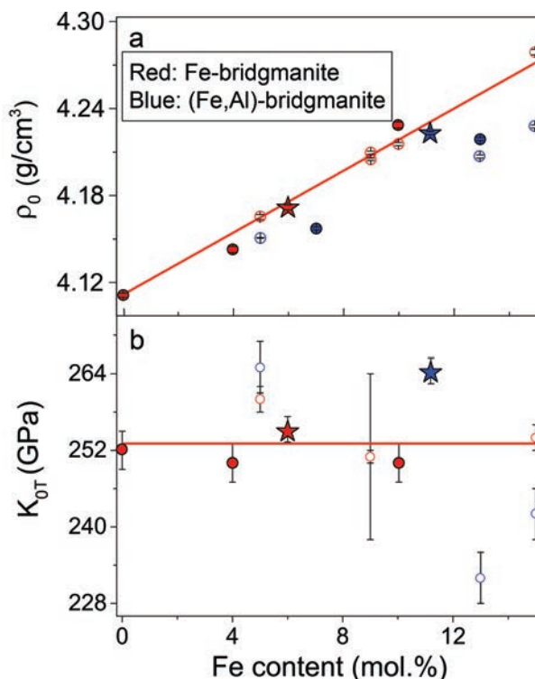
FIGURE 7. Density ( \rho_0 ) and bulk modulus ( K_{0T} ) of bridgmanite at ambient conditions. (a). \rho_0 ; (b). K_{0T} . Red = Fe-bearing bridgmanite; blue = (Fe,Al)-bridgmanite; open symbols = results from polycrystalline bridgmanite samples (Andraut et al. 2001; Catalli et al. 2010, 2011; Dorfman et al. 2013; Lundin et al. 2008; Mao et al. 1991); solid symbols = results from single-crystal bridgmanite samples (this study; Boffa Ballaran et al. 2012; Saikia et al. 2009); stars = our Bm6 and Al-Bm11. Errors are smaller than symbols when not shown. (Color online.)
