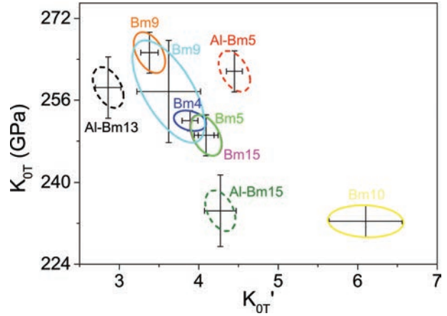
FIGURE 8. Confidence ellipses of the bulk modulus ( K_{0T} ) and its pressure derivative ( K'_{0T} ) of bridgmanite at ambient conditions at the 1\sigma level using literature data. Solid lines = Fe-bearing bridgmanite; dashed lines = (Fe,Al)-bridgmanite; Blue = Bm4 (Boffa Ballaran et al. 2012); green = Bm5 (Andraut et al. 2001); orange = Bm9 (Lundin et al. 2008); light blue = Bm9 (Dorfman et al. 2013); yellow = Bm10 (Mao et al. 1991); magenta = Bm15 (Lundin et al. 2008); red = Al-Bm5 (Andraut et al. 2001); black = Al-Bm13 (Catalli et al. 2011); olive = Al-Bm15 (Nishio-Hamane et al. 2009). (Color online.)
