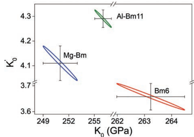
FIGURE 5. Error ellipses of K_{0T} - K'_{0T} for Bm6 and Al-Bm11 at the 1 \sigma level. Red = Bm6; green = Al-Bm11; blue = Mg-Bm (Boffa Ballaran et al. 2012). (Color online.)
