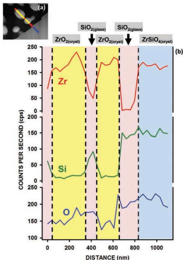
FIGURE 3. Variation in Si, Zr, and O along a traverse on Zr09. The corresponding phase identities have been inset. X-ray fluorescence spectra taken with TEM operating in STEM mode. Intensity variation corresponds to band intensities for Zr ( L\alpha , 2.04 keV), Si ( K\alpha , 1.74 keV), and O ( K\alpha , 0.53 keV).
