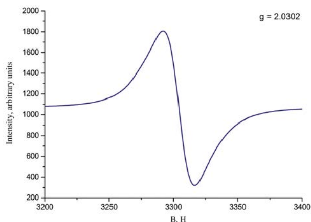
FIGURE 6. EPR spectrum of S-rich lazurite at room temperature.
