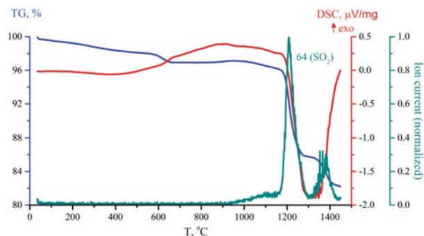
FIGURE 2. Thermogravimetric (TG) and differential scanning calorimetry (DSC) curves and the temperature dependence of the \text{SO}_2 ion current (mass number 64) for lazurite sample 1.
