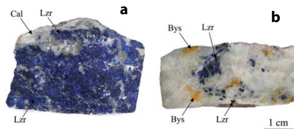
FIGURE 1. Samples of rocks with high-sulfur lazurite: (a) lenticular body (sample 1), (b) lazurite-containing calciphyre with bystrite (sample 2). Abbreviations: Lzr = lazurite, Bys = bystrite, Cal = calcite.
