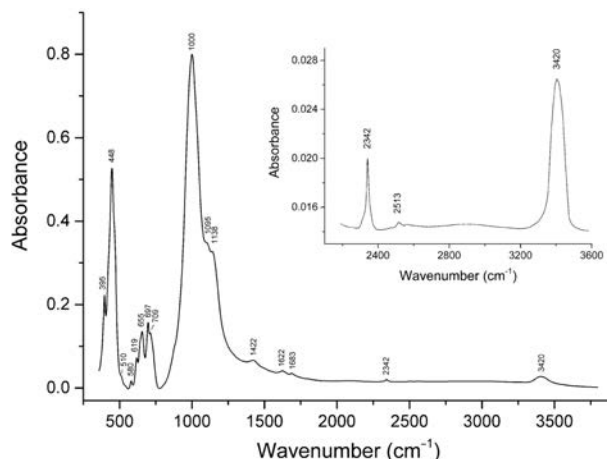
FIGURE 4. Infrared absorption spectrum of S-rich lazurite (sample 1).
