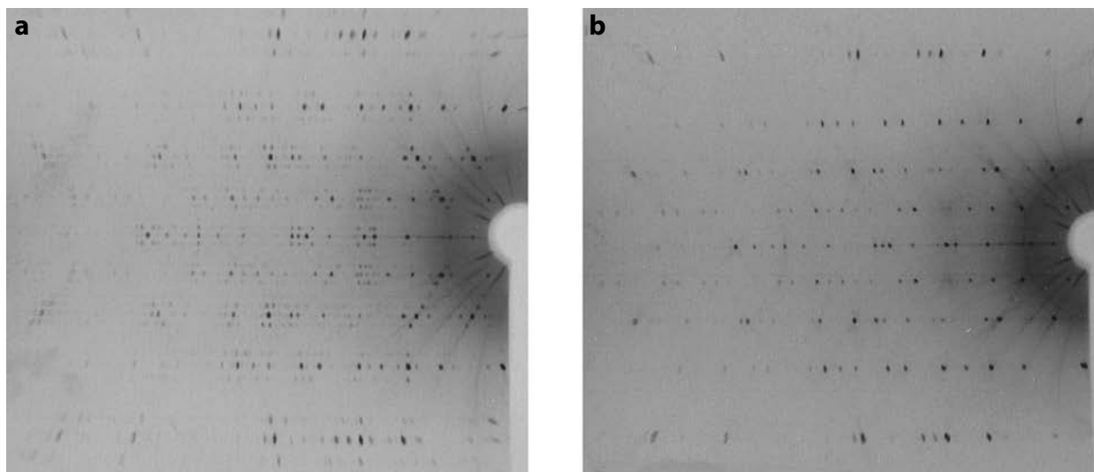
FIGURE 7. Single-crystal X-ray rotation photographs of lazurite ( a = 9.071 Å and n = 0.218 ): initial crystal of lazurite with (a) incommensurate modulation reflections and (b) crystal annealed at 650 °C in air for 1 h, without incommensurate modulation reflections.
