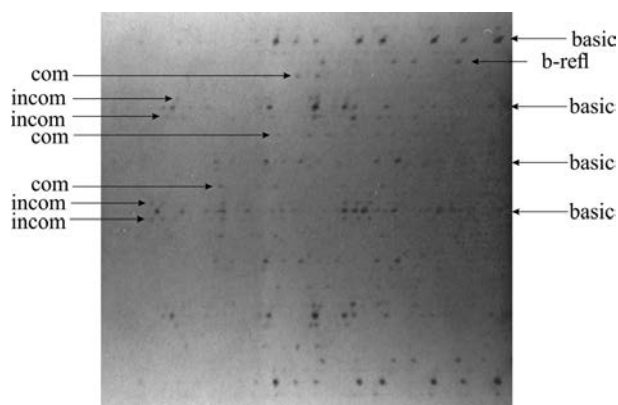
FIGURE 8. The [100] single-crystal X-ray rotation photograph of S-rich lazurite (sample 1). basic = reflections of the subcell; com = commensurate modulation; incom = incommensurate modulation; and \beta -refl = \beta -reflections are indicated.
