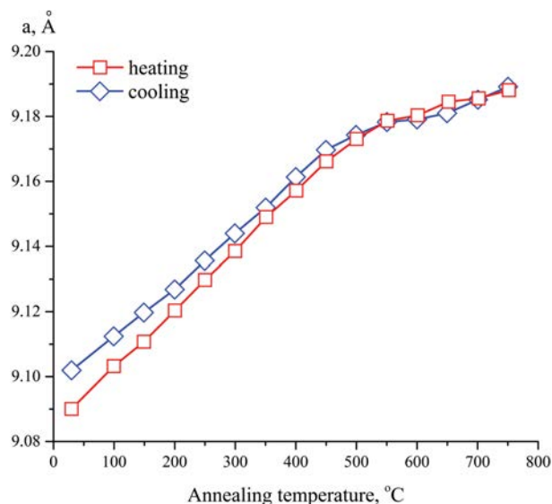
FIGURE 9. Dependence of the sub-cell parameter of S-rich lazurite on temperature.
