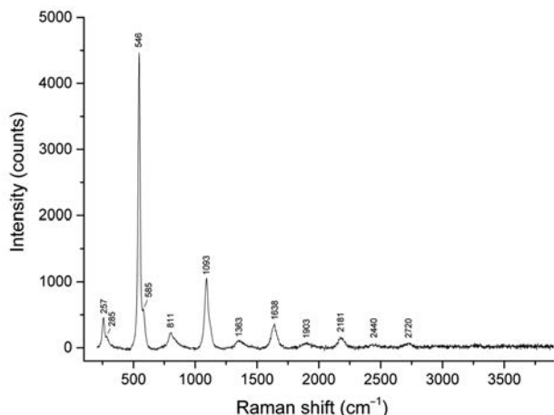
FIGURE 3. Raman spectrum of S-rich lazurite (sample 1).
