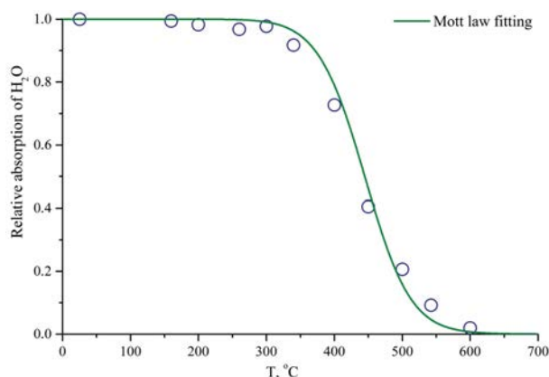
FIGURE 5. Temperature dependence as a function of relative intensity of IR absorption at 3400 cm -1 (stretching vibrations of H 2 O molecules).
