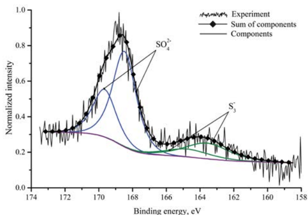
FIGURE 10. S 2p XPS spectra of the dark blue lazurite from the Malo-Bystrinskoe deposit. The peak parameters are given in Table 6.
