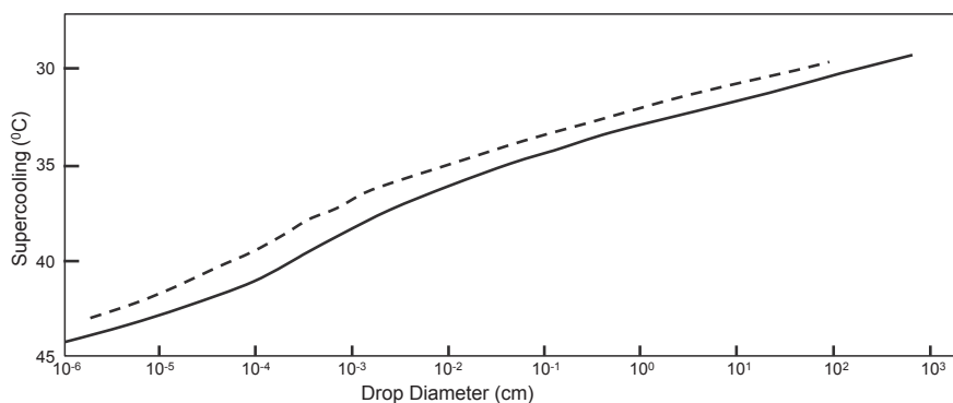
Figure 6. The relationship between the supercooling required to crystallize ice from ultra-pure water, as a function of the drop diameter. The full line is for a cooling rate of 1\ ^{\circ}\text{C}\ \text{s}^{-1} and the dashed line for a cooling rate of 1\ ^{\circ}\text{C}\ \text{min}^{-1} . The data for the lines are from a large number of experiments analyzed by Prupacher (1995).
