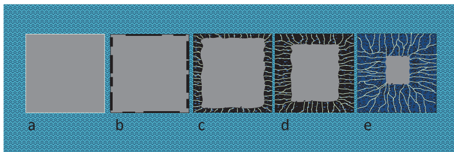
Figure 2. Schematic drawing of a pseudomorphic replacement reaction. When a solid (a) is out of equilibrium with an aqueous solution, it will begin to dissolve. The resulting fluid composition at the interface with the solid may become supersaturated with respect to another phase and (b) precipitate on the surface of the dissolving solid. This sets up a feedback between dissolution and precipitation. For the dissolution–precipitation reaction to continue (c–e), the precipitated phase must have interconnected porosity, allowing fluid access to the reaction interface and diffusion of components through the fluid
