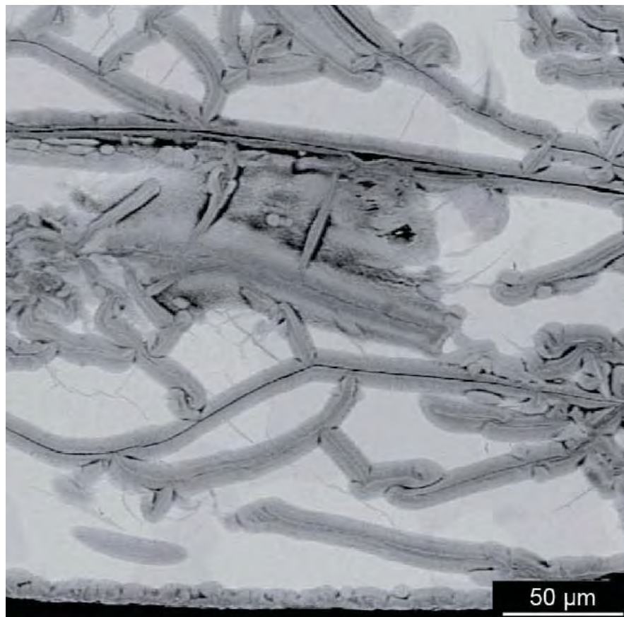
Figure 4. A back-scatter electron (BSE) image of a cross-section through an ilmenite crystal ( \text{FeTiO}_3 ) partly replaced by an Fe-poor phase, which eventually results in the whole crystal being replaced by rutile. The “leaching” of the Fe from the ilmenite takes place by the generation and propagation of fractures (dark) through the unaltered ilmenite and precipitation of rutile from the fluid in the fractures. (See Janssen et al. 2010).
