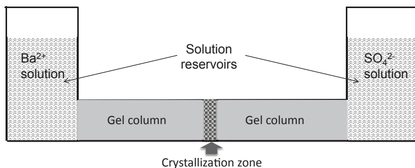
Figure 7. Schematic of the experimental set-up for double diffusion crystal growth experiments where a gel column separates the reacting components, in this case \text{Ba}^{2+} and \text{SO}_4^{2-} . Counter-diffusion of the components through the gel column eventually supersaturates the fluid and results in precipitation (of \text{BaSO}_4 in this case).
