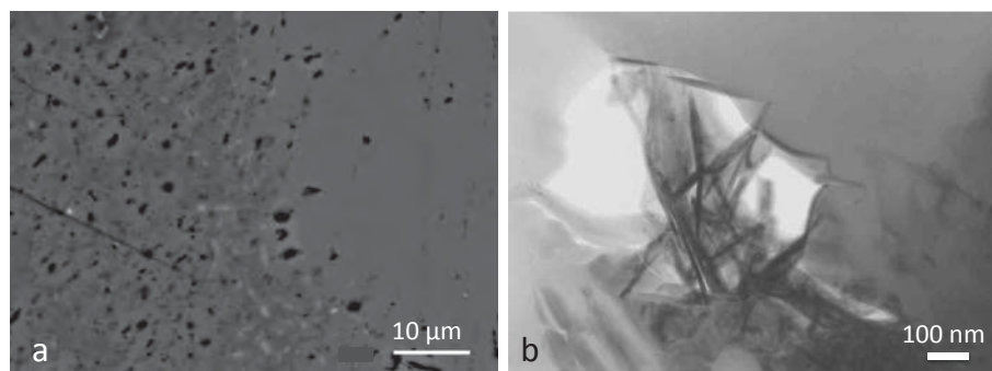
Figure 3. (a) A back-scatter electron (BSE) image of an albitization reaction front in a plagioclase single crystal from partly albitized rock in the Bamble Sector, south Norway. The smooth textured phase on the right is the parent oligoclase and the darker phase on the left is the product albite. The black spots in the albite are pores. The lighter laths are sericite. (b) During replacement of feldspars hematite may crystallize within the pore-spaces, giving the rock a reddish color, such as commonly seen in pink granites.
