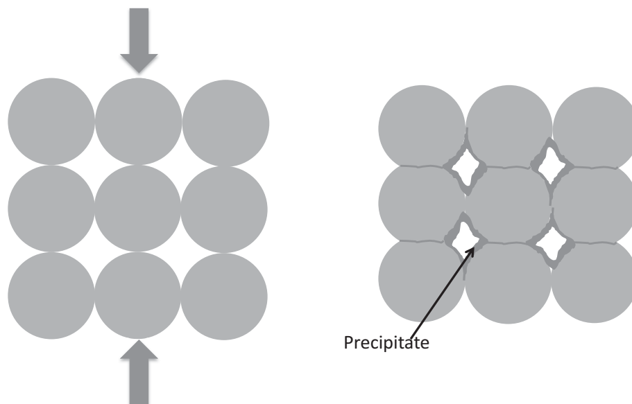
Figure 1. Schematic drawing of pressure solution. A material under applied stress dissolves at the stress points, where the spherical grains are in contact, and is transported through the solution to sites of lower stress where it reprecipitates. Compaction by pressure solution reduces the porosity and permeability of a rock.
