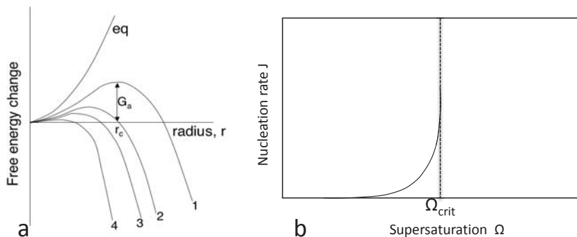
Figure 5. (a) Schematic drawing of the change in free energy as a function of nucleus size according to classical nucleation theory (CNT). The curve “eq” represents the free energy of a particle formed at equilibrium where only a surface energy term would be relevant. Curves (1) to (4) show the situation with increasing supersaturation where the reduction in free energy is dominated by the volume free energy of the nucleus. (b) A consequence of CNT is that the nucleation rate is a very sharp function of the supersaturation and defines an approximate value of the critical supersaturation for nucleation.
