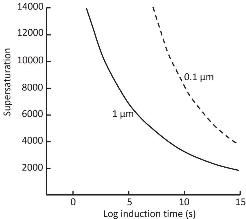
Figure 9. Calculated curves from CNT for the relationship between the supersaturation and the induction time for nucleation in pores of size 0.1 \mu\text{m} and 1 \mu\text{m} (after Prieto 2014).
