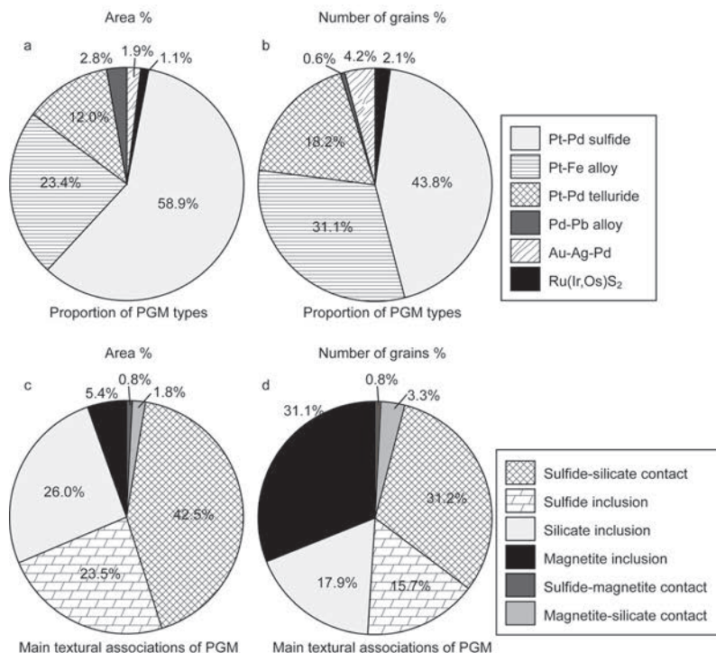
Figure 6. Pie charts illustrating the proportion of PGM observed in the four samples from the J-M Reef (troctolite, anorthosite, leuconorite, and olivine melagabronorite with ~1 to ~5 vol.% base-metal sulfides) studied by Godel and Barnes (2008b) by area (a) and number of grains (b). The samples contain ~49 to 419 ppm bulk rock PGE (see also Fig. 2). Summary pie charts of the textural distribution of the different PGM by (c) area and (d) number of grains have been replotted using the data presented in Figures 3 and 4 of Godel and Barnes (2008b).
