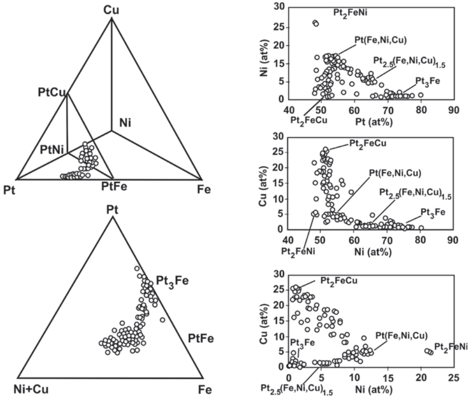
Figure 18. Compositional variation of Pt-alloys hosted in chromites from the concentrically zoned complexes of the Urals (Kytlym and Uktus). These plots are adapted, replotted and redrawn from Garuti et al. (2002).
