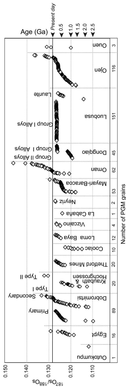
Figure 12. ^{187}\text{Os}/^{188}\text{Os} isotopic ratios and corresponding T_{\text{RD}} model ages for PGM analyzed in situ in chromitites from ophiolite-type ultramafic complexes; updated after González-Jiménez et al. 2014a. Data sources: Coolac Serpentine Belt, Australia (Belousova et al. 2015); Dobromiritsi (Bulgaria; González-Jiménez et al. 2013a, 2014c); Eastern Desert, Egypt (Ahmed et al. 2006); Hochgrössen and Kraubath massifs, Austria (Malitch 2004; Malitch et al. 2003); La Cabaña (this study); Loma Baya, Guerrero State, Mexico (González-Jiménez et al. 2014b); Luobusa and Dongqiao, Tibet (Shi et al. 2007; McGowan et al. 2015); Mayari-Baracoa, eastern Cuba (Marchesi et al. 2011; González-Jiménez et al. 2012a); Neyritz (this study); Ojén (González-Jiménez et al. 2013a); Ouen Island (González-Jiménez et al. 2014b); Outokumpu ophiolite, Finland (Walker et al. 1996); Theftord Mines, Canada (this study); Vizcaino, California State, Mexico (this study).
