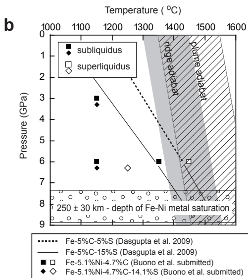
(b) P - T diagram showing the experimental constraints on the liquidus of Fe-C-S (Dasgupta et al. 2009a) and Fe-Ni-C \pm S (Buono et al. submitted) bulk compositions shown in (a). Shown for comparison in (b) are the mantle adiabats relevant for MORB and OIB production, i.e., ridge adiabat and plume adiabat, respectively. Also shown for reference is the minimum depth where Fe-Ni alloy saturation is thought to occur according to the study of Rohrbach et al. (2011). Comparison between the liquidi of the metallic compositions and the adiabats suggests that, especially for S-bearing and S-rich compositions, the deep upper mantle may contain a sulfide-rich Fe-Ni-C-S metallic liquid phase and solid carbide stability may require somewhat greater, perhaps transition zone depths.
