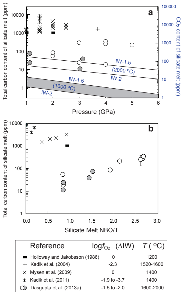
Figure 4a,b. Storage capacity of carbon in silicate magma at core-forming conditions ( f_{\text{O}_2} \sim\text{IW}-4 to \text{IW} ), modified after Dasgupta et al. (2013a). (a) Total carbon content in silicate melts as a function of pressure. A range of silicate compositions saturated with \text{CH}_4 - \text{H}_2 fluid and/or graphite and at temperatures of 1200-2000 °C is plotted. Also shown for reference are the \text{CO}_2 solubilities in a tholeiitic basalt at graphite saturation at 1600 and 2000 °C and between f_{\text{O}_2} similar to IW-2 to IW-1.5, following the model of Holloway (1992). (b) Estimated concentration of total dissolved carbon in silicate melt as a function of melt depolymerization index NBO/T (Mysen 1991) for the studies plotted in (a).
