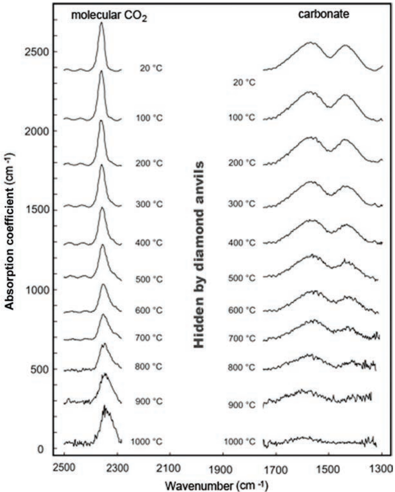
Figure 17. High-temperature in situ FTIR spectra of dacite melt with 1.6 wt% CO 2 . Pressure increases from 5 GPa at room temperature to 14 GPa at 1000 C. Spectra were measured at the synchrotron source ANKA in Karlsruhe, Germany. After Korschak (2008).
