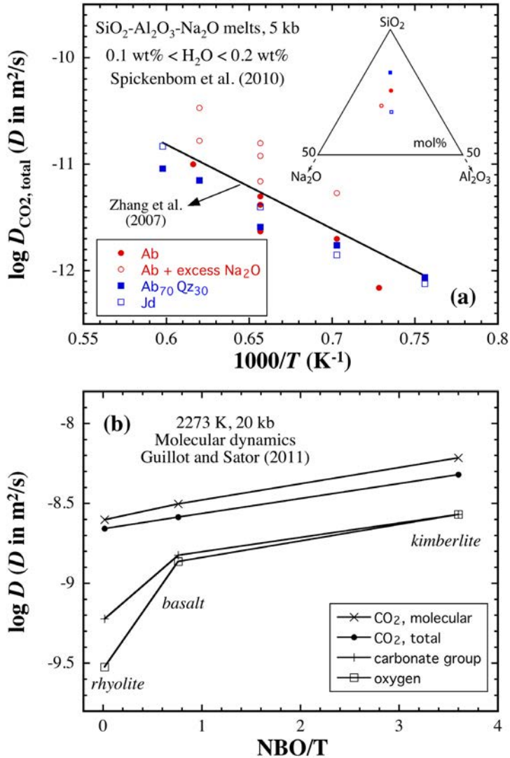
Figure 22. (a) Experimental total \text{CO}_2 diffusivity at 0.5 GPa in four anhydrous ( \text{H}_2\text{O} ranging from 0.1 to 0.2 wt%) \text{SiO}_2\text{-Al}_2\text{O}_3\text{-Na}_2\text{O} melts with the inset showing the loci of melts in compositional space. Modified after Spickenbom et al. (2010). Calculations using the composition-independent model of Zhang et al. (2007) at 0.15 wt% \text{H}_2\text{O} are shown for comparison (solid line). (b) Molecular dynamics-derived diffusivity of total \text{CO}_2 , molecular \text{CO}_2 , \text{CO}_3^{2-} , and oxygen versus \text{NBO}/\text{T} of three melts at 2273 K and 2.0 GPa. After Guillot and Sator (2011).
