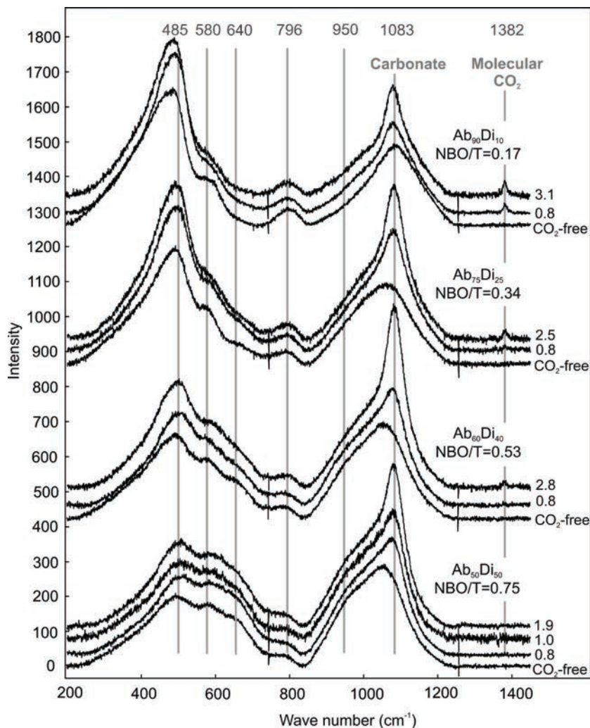
Figure 14. Raman spectra of some CO 2 -bearing glasses along the albite (NaAlSi 3 O 8 ) - diopside (CaMgSi 2 O 6 ) join. For each glass composition, spectra with different bulk CO 2 content (in wt%) are shown. After Korschak (2008).
