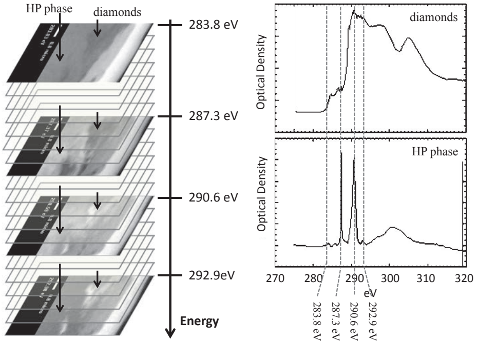
Figure 9. Left: STXM stacks of transmitted images (processed into optical density images) taken at 0.1 eV energy intervals, from which spectra can be extracted for each area. Right: Spectra for one area containing the high-pressure (HP) phase, corresponding to a new phase of \text{FeCO}_3 . Spectra from a different area containing to nanodiamonds is shown at top.
