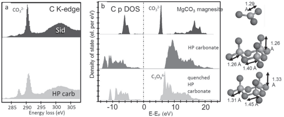
Figure 7. (a) Carbon K-edge spectra collected from a recovered sample of Fe-bearing magnesite compressed and heated to 80 GPa and 2300 K in the untransformed (top spectra) and transformed (bottom spectra) areas; (b) DFT calculations for electron density of state of the carbon atoms ( p orbital symmetry) in different structures (schematics shown at right). This unoccupied density of state roughly corresponds to the excitation probed by EELS at the carbon K-edge (excitonic effects are neglected in the calculation). Modified after Boulard et al. (2011).
