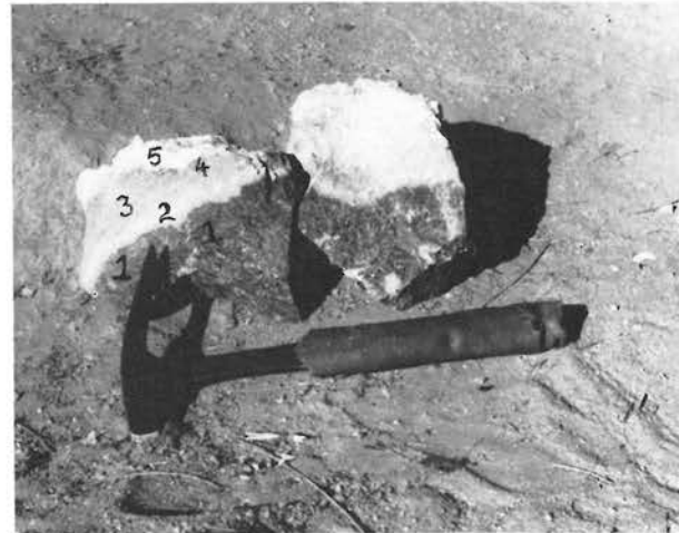
FIG. 3. Specimens from druses in a well along section AB. 1 to 5 zones in the specimen.
