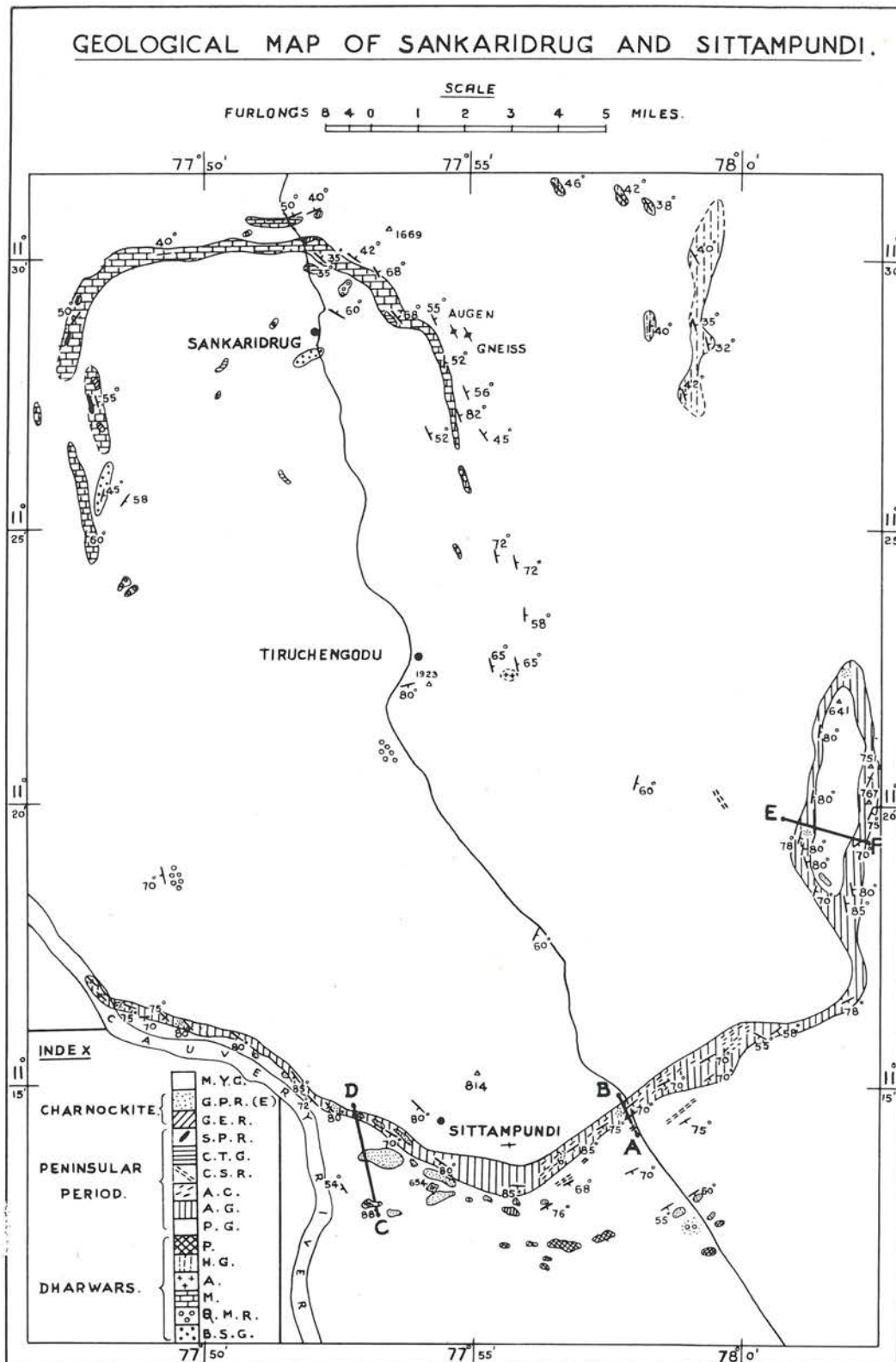
FIG. 1. Geological map of Sankaridrug and Sittampundi. In the index, M.Y.G.—Migmatite and younger granite. G.P.R.(E)—Garnet-pyroxene rock (eclogite). G.E.R.—Garnet-epidote rock. S.P.R.—Scapolite-pyroxene rock. C.T.G.—Calc-tremolite gneiss. C.S.R.—Calc-silicate rock. A.C.—Amphibolite with chromite. A.G.—Anorthite gneiss. P.G.—Peninsular gneiss (not mapped separately from younger granite). P—Peridotite. H.G.—Hornblende gneiss. A—Amphibolite. M—Marble. Q.M.R.—Quartz-magnetite rock. B.S.G.—Biotite-sillimanite gneiss. AB, CD and EF are sections along the anorthite gneiss band.
