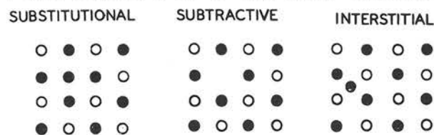
FIG. 1. Types of defects in a diatomic crystal.
