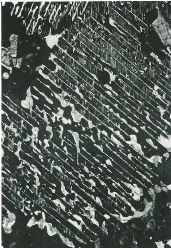
FIG. 12. A former pigeonite grain contained within a much larger ferropyrroxene grain; the outline of the pigeonite grain is delineated by the relict hedenbergite exsolution lamellae which had developed parallel to (001). The thinner, near vertical striations are hedenbergite exsolution lamellae that are parallel to (100) in the ferropyrroxene. Note that in part of the grain the later (100) lamellae are missing and in that part of the grain the (001) lamellae are characterized by conspicuous protuberances. (Crossed nicols, \times 56 ).
