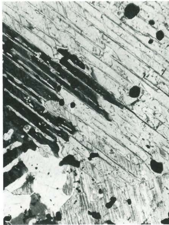
FIG. 13. Part of a former pigeonite grain in which hedenbergite exsolution lamellae had developed parallel to (001). The boundary between two adjacent ferropyrroxene grains cuts through the region occupied by the former pigeonite, disregarding the previous grain boundaries. Note that the hedenbergite lamellae extend across this grain boundary. The near vertical striations in the righthand grain are hedenbergite exsolution lamellae that are parallel to (100) of the ferropyrroxene. (Crossed nicols, \times 72 ).
