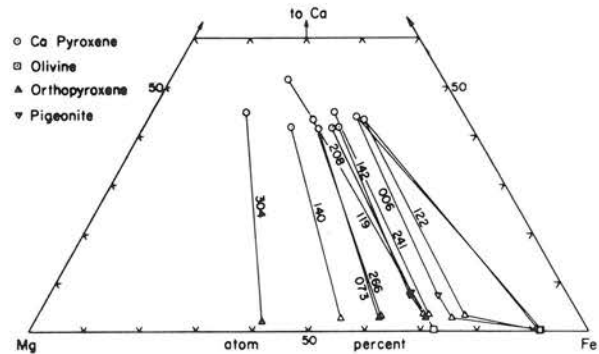
FIG. 6. Orthopyroxenes and olivines coexisting with Ca pyroxenes. Also shown are the initial compositions of the inverted pigeonites in samples 006, 142 and 208. Orthopyroxene is not present in sample 119 and quartz is not present in samples 119 and 142.
