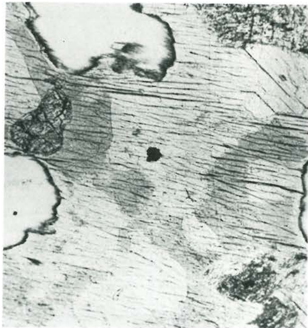
FIG. 19. A portion of a cummingtonite grain that varies from colorless and well-twinned (light grey) to untwinned and pleochroic in various shades of green (medium grey). Small remnants of altered Ca pyroxene (high relief) are present within the cummingtonite and acicular cummingtonite fibers have grown at the edges of the quartz. (Plane light, \times 64 )
