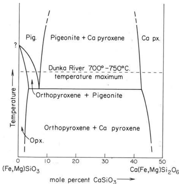
FIG. 8. Proposed temperature-composition relationships among iron-rich Ca pyroxene, pigeonite, and orthopyroxene. This figure is a section across the pyroxene quadrilateral through the fields of Ca pyroxene, pigeonite, and orthopyroxene approximately along the tie line in the Ca pyroxene-pigeonite field of Figure 7.
