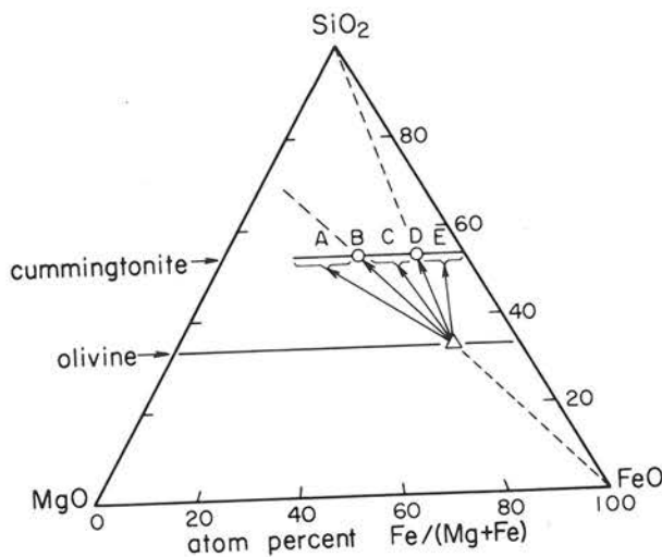
FIG. 26. Graphical representation of some possible reactions for fayalite that has a specific composition being replaced by cummingtonites of various compositions. See text for reactions and explanation.
