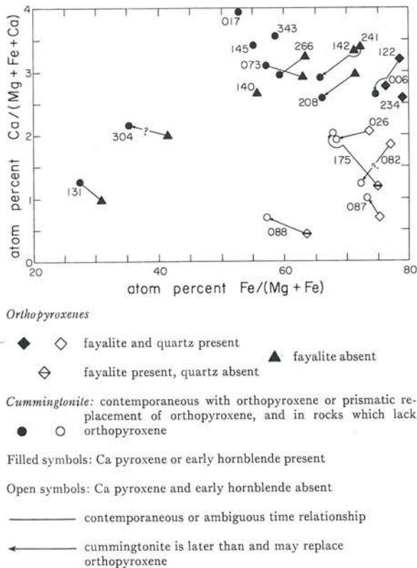
FIG. 4. Compositions of orthopyroxenes and cummingtonites from the Dunka River area. Orthopyroxenes 006, 122, 142 and 208 are inverted from pigeonite.
