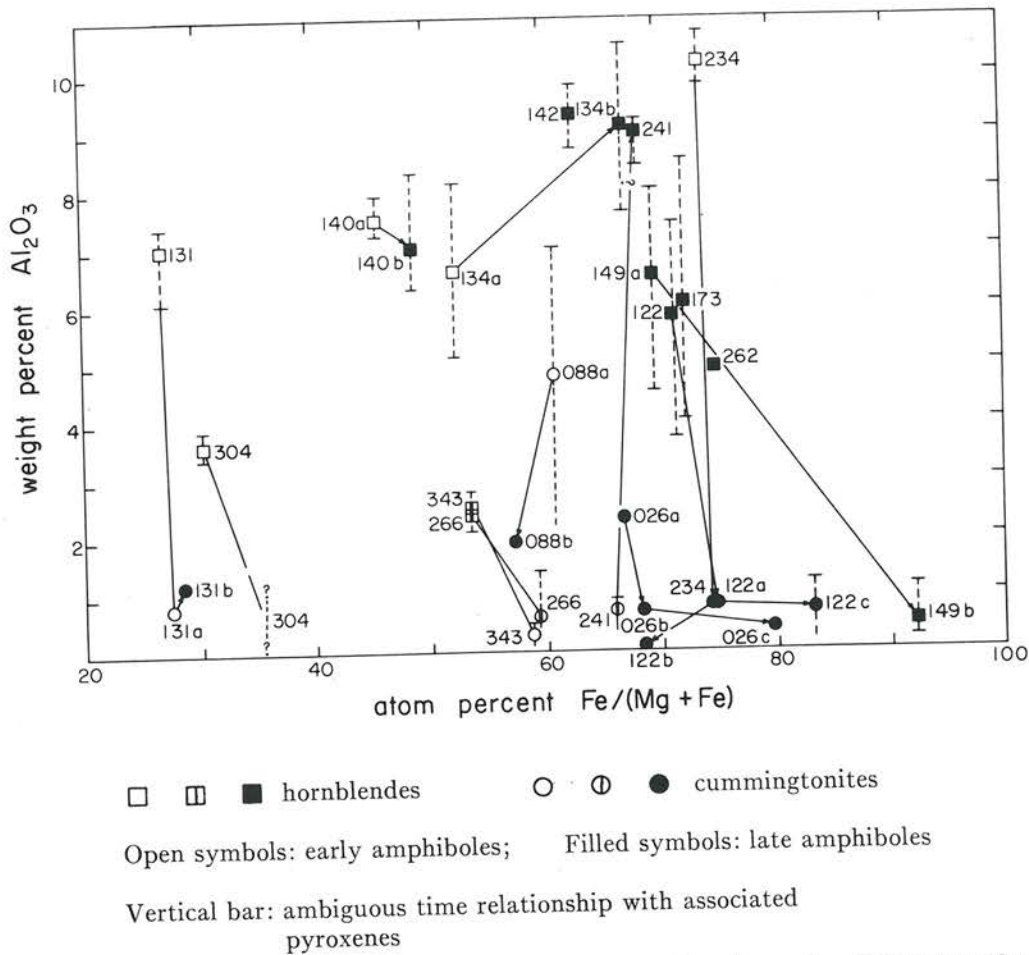
FIG. 22. Plot of weight % Al_2O_3 versus atom % Fe/(Mg+Fe) for cummingtonites and hornblendes from the Dunka River area. Arrowheads on the ends of some tie lines indicate the sequence of formation. The range of Al_2O_3 % in hornblende from an individual rock is indicated by the vertical dashed line. Cummingtonite is present in sample 304, however its Al_2O_3 content was not measured. Sample 149(b) is a late acicular ferroactinolite overgrowth on hornblende grains.
