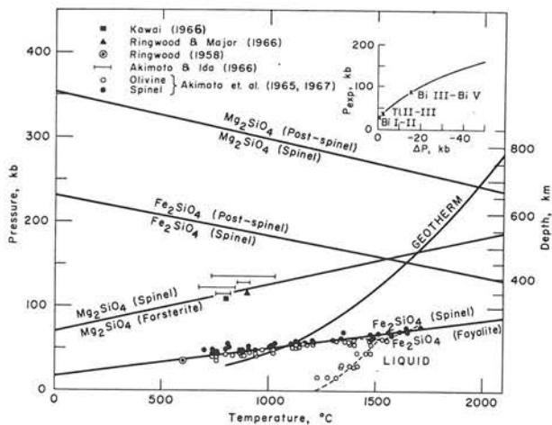
FIG. 3. Stability fields of forsterite and fayalite and a representative geotherm.
