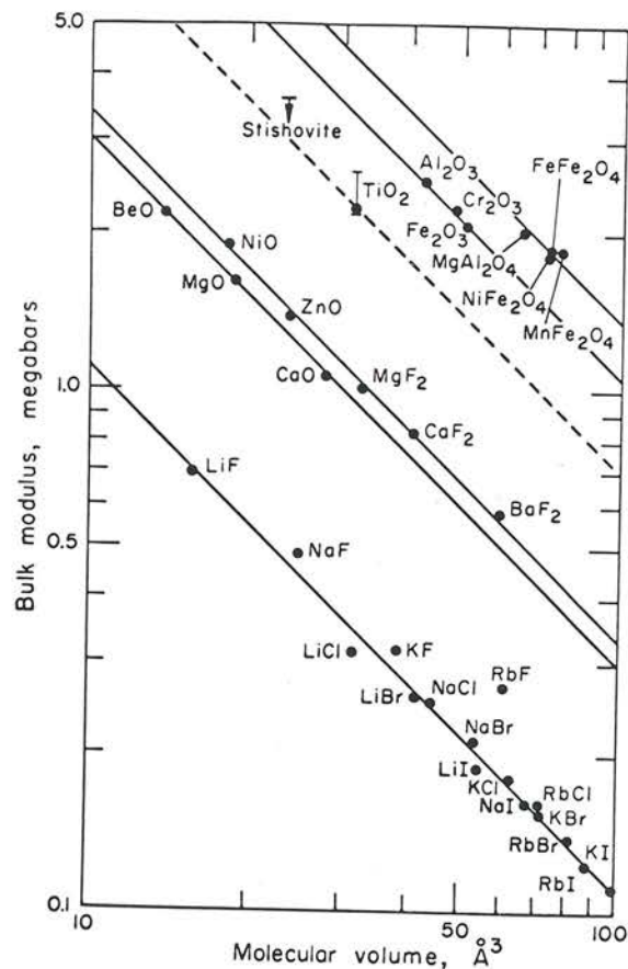
FIG. 13. Bulk modulus vs. molecular volume for halides and oxides after Anderson and Anderson (1970).
