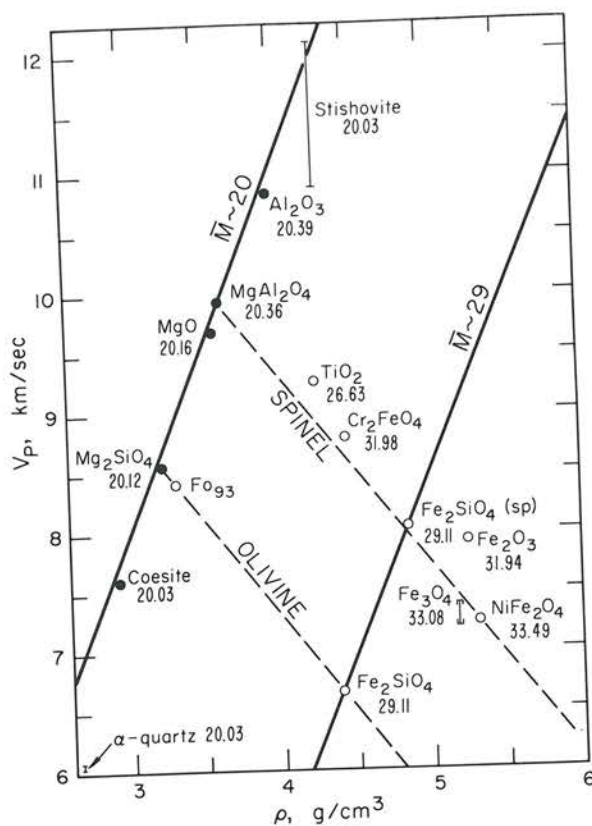
FIG. 11. Compressional velocity vs. density for oxides and silicates. Data from Anderson et al. (1968), Mitzutani et al. (1970) and Lieberman ( pers. commun. )
