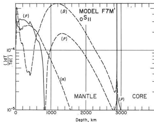
FIG. 7. Free oscillation variational parameters for spheroidal mode {}_0S_{11} showing the importance of density, \rho , in the upper mantle. For this mode the most important parameter is shear velocity \beta , in the middle mantle and this is determined from body wave studies. Most of the modes of free oscillation are not very sensitive to the compressional velocity, \alpha .
