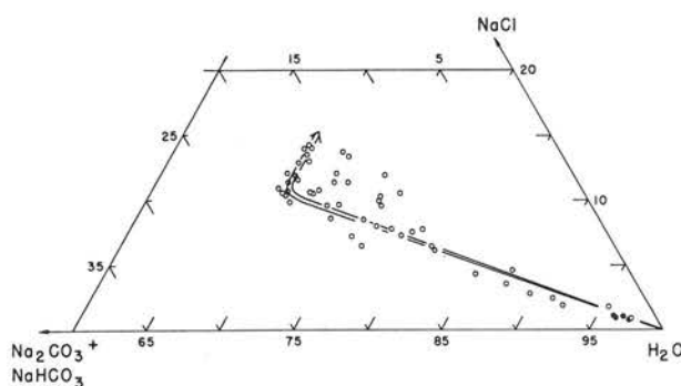
FIG. 16. Magadi hot springs and brines in the system (\text{NaHCO}_3 + \text{Na}_2\text{CO}_3)\text{-NaCl-H}_2\text{O} . Dots are hot springs, circles are lagoon, surface, interstitial and core hole brines. The path shown is the evaporative trend with NaCl enrichment due to the precipitation of trona.
