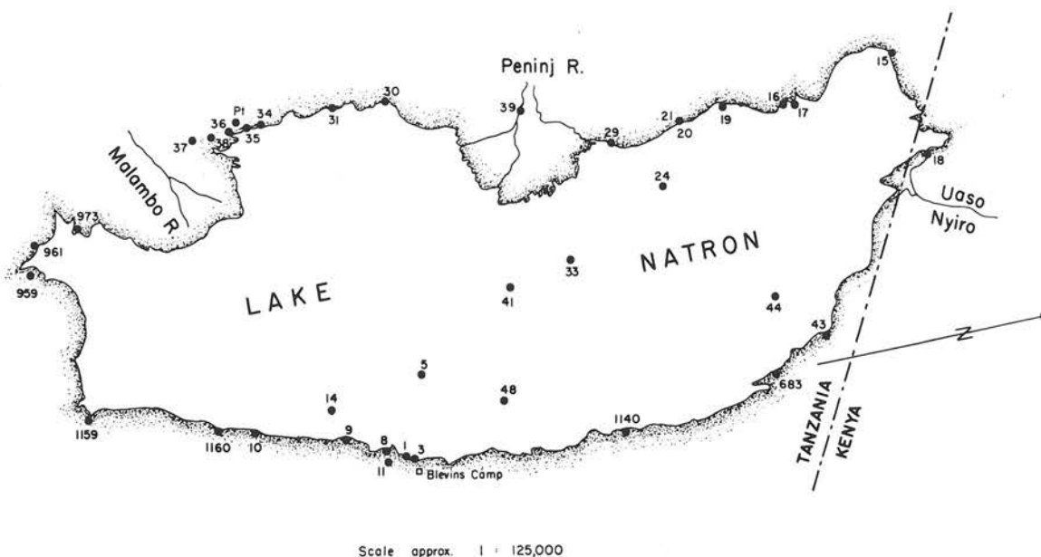
FIG. 21. Sampling stations for Lake Natron (simplified from Guest and Stevens, 1951). The numbers are identified in Table 4.
