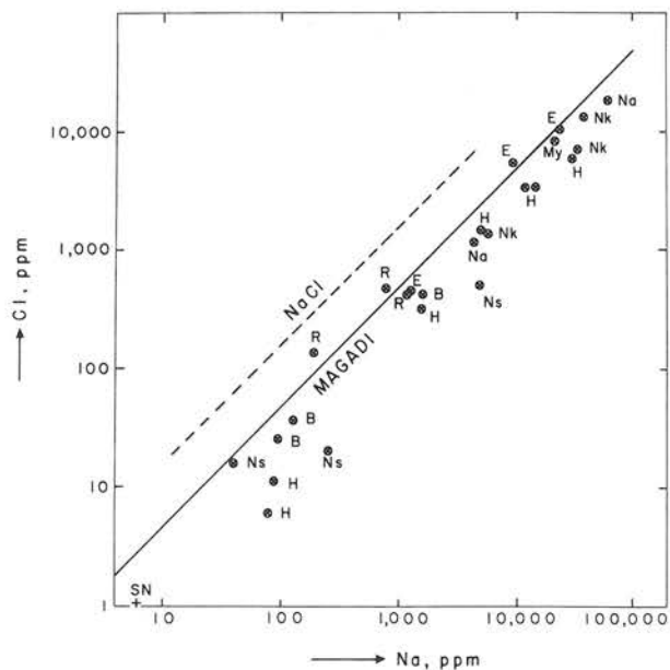
FIG. 14. Chloride versus sodium for East Rift Valley lakes. For key to abbreviations see Fig. 1. Solid line is for Magadi trend, from Fig. 4. Dashed line is for Na:Cl (equal molalities). Data from Talling and Talling (1965).
