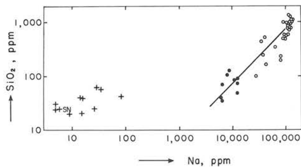
FIG. 13. Silica versus sodium. Symbols as in Fig. 4.
