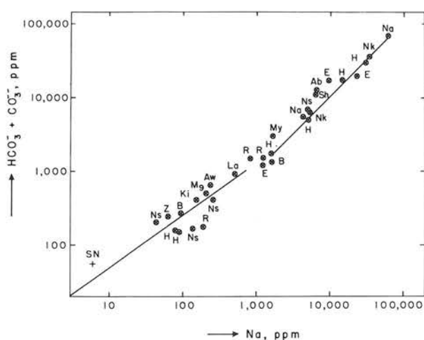
FIG. 15. Total carbonate versus sodium for East Rift Valley lakes. For key to abbreviations see Fig. 1. Solid lines are for Magadi, from Fig. 7.
