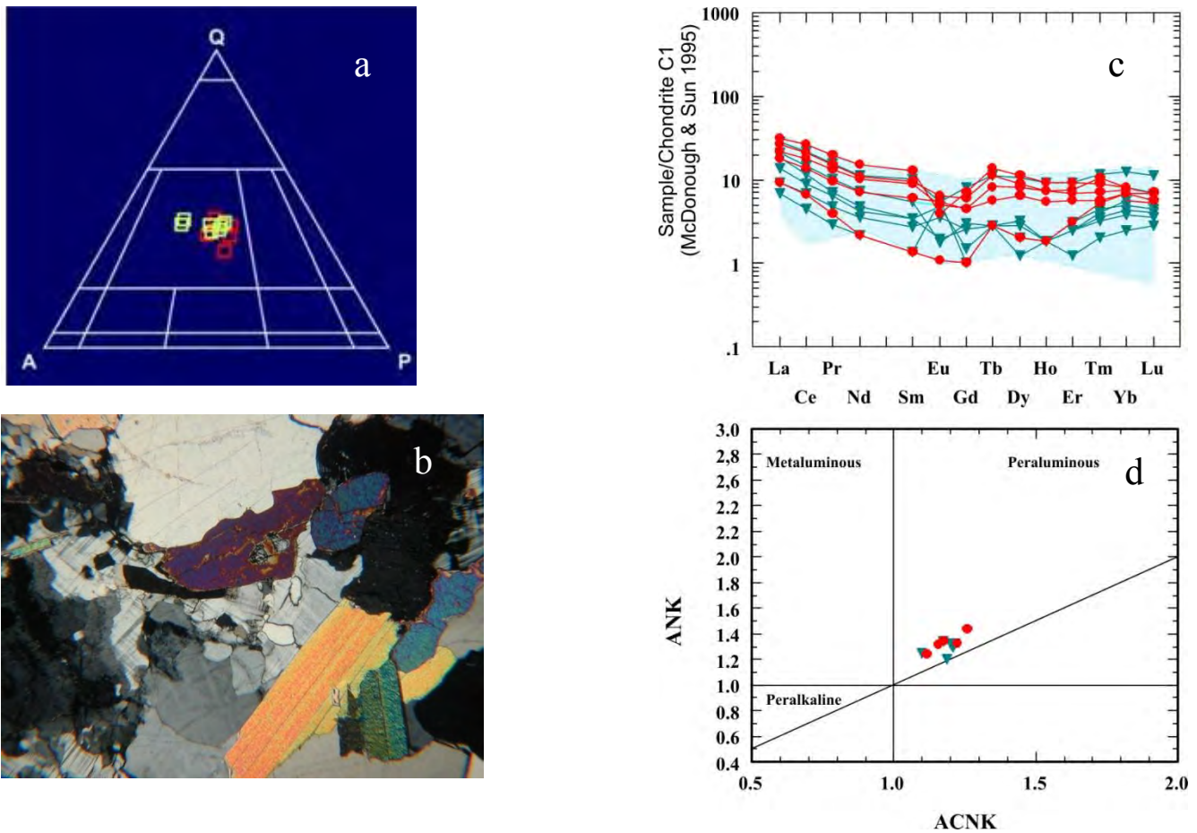
Figure 4a: Modal composition of the Paso del Rey leucogranite plotted in the QAPF triangular diagram, yellow squares correspond to medium-grained samples, red squares to pegmatitic facies; 4b: photomicrograph of a tourmaline-muscovite leucogranite of Paso del Rey; 4c: REE diagram with the samples of Paso del Rey and Cerro La Torre leucogranites (red and bluish respectively) with the domain of Harney Peak granites after Nabelek & Liu (2004); 4d: ASI index in the diagram for the considered leucogranites.
