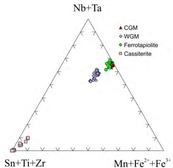
Figure 30: Triangular diagram showing the composition of the Nb-Ta-Sn-Ti ore minerals
