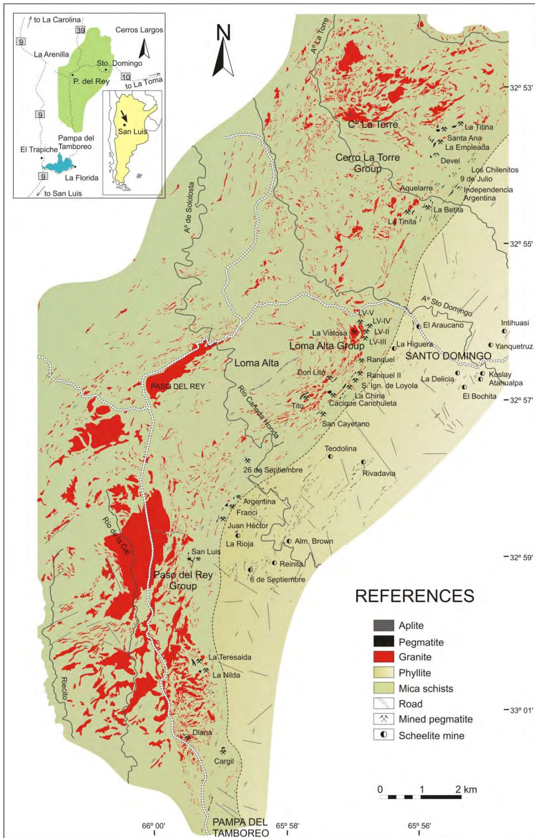
Figure 3: Geological map of the El Totoral pegmatite field showing the distribution of the different pegmatites and their parental leucogranites (modified from Oyarzábal et al. 2009).
