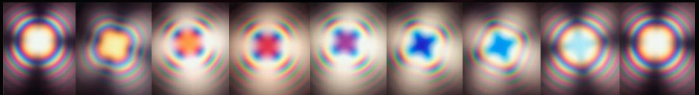
Figure 1. The “bull’s eye” uniaxial optic figure characteristic of quartz is indicative of its optical activity. This is the view seen looking directly along the optic axis of the crystal when viewed between two crossed polarizing filters in transmitted white light - that is, looking towards the light source. The N-S, E-W dark areas are the remnants of isogyres which in uniaxial minerals normally form a black cross in the center, but which in slices thicker than 1 mm are extinguished by quartz’s strong optical activity and low birefringence, thus forming the bull’s eye appearance. The outer rings of color are isochromes and follow those of Newton’s Rings. The central colors recombine with increased thickness and ultimately leave only a red changing to green sequence in the center. Rotating the filter farthest from the light source in a clockwise direction for 180 degrees cycles the bull’s eye through a series of colors and shapes that depend on thickness . For this 3.0 mm basal slice, the left to right sequence of changing colors indicates that it is likely an optically left-handed quartz; confirmed with observation using a quarter-wave plate as seen in Figure 5 or by direct measurement with monochromatic light as seen in Figure 11.
