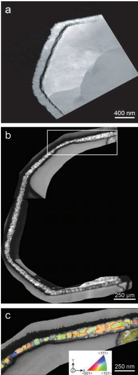
Figure 10. (a) TEM high angle annular dark field (HAADF) image of a diamond FIB foil showing a pyrrhotite inclusion with a magnetite rim. (b) Foreshooter electron image of the magnetite corona. (c) Crystal preferred orientation of magnetite in the area indicated by a white rectangle in (b) color-coded according to the legend and the reference frame ( bottom right ). Grain boundaries are in black , red lines are twin boundaries. Modified after Jacob et al. (2016).
