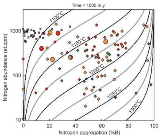
Figure 6. Variation diagrams for the average degree of nitrogen aggregation (%) vs. nitrogen abundance (at. ppm) for the diamonds from PDAs ( circles ) alongside the fibrous ( squares ) and monocrystalline diamonds ( diamonds ) from Orapa (adapted from Mikhail et al. 2019b). Isotherms chart the residence times of 1000 m.y. using the DiaMap software (Howell et al. 2012a, b). Red symbols—eclogitic paragenesis, green —peridotitic, blue —websteritic, grey —fibrous unknown, orange —unknown.
