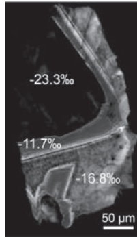
Figure 4. Cathodoluminescence image of a diamond fragment from a websteritic PDA from Venetia showing different growth zones with variable \delta^{13}\text{C} values, indicating different growth pulses.
