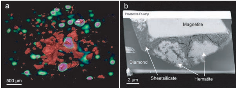
Figure 2. (a) \mu CT region of interest showing pore space (red) and magnetite grains (purple) covered by a replacement envelope (green) of a mixture of hematite and a sheet silicate. Diamonds are rendered transparent in this view. (b) TEM HAADF image of a FIB foil cut from a diamond grain showing a replacement rim around magnetite consisting of a mixture of hematite and a sheet silicate.
