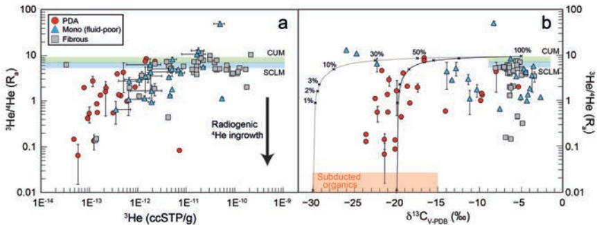
Figure 5. Helium isotope systematics of fluids released by in vacuo crushing and heating of PDAs, and monocrystalline and fibrous diamonds. The ^3\text{He}/^4\text{He} and \delta^{13}\text{C} value of the modern convecting upper mantle (CUM) and the sub-continental lithospheric mantle (SCLM) are shown for reference (adapted from Mikhail et al. 2019a). The mixing lines shown in (a) are drawn between oceanic crustal-derived fluids with \delta^{13}\text{C} = -20 and -30\text{‰} , and ^3\text{He}/^4\text{He} = 0.01 Ra, and mantle-derived fluids with \delta^{13}\text{C} = -5\text{‰} and ^3\text{He}/^4\text{He} = 9 Ra. The mixing lines plotted in (b) are hyperbolic as [\text{He}]_{\text{mantle}}/[\text{He}]_{\text{crust}} is assumed to be 10. Note, the mantle ^3\text{He}/^4\text{He} endmember is slightly higher than the present-day upper asthenosphere and lithosphere mantle value, reflecting the U–Th decay-driven temporal evolution of ^3\text{He}/^4\text{He} in the silicate Earth (Porcelli and Elliott 2008). Therefore, all ^3\text{He}/^4\text{He} ratios are minimum values, although it appears that diamonds with >1 \times 10^{-12} ccSTP ^3\text{He}/\text{g} are largely immune to the effect of ingrowth because the ^4\text{He} production is too low to offset the R/Ra in this system (note the logarithmic scale of the x-axis). Comparative data are from Burgess et al. (1998), Gautheron et al. (2005), Broadley et al. (2018), Timmerman et al. (2018, 2019a, b), and Mikhail et al. (2019a).
