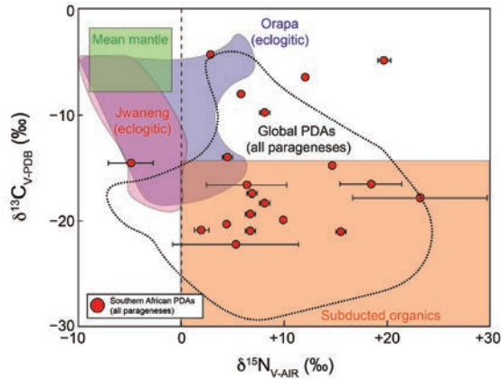
Figure 3. Plot of \delta^{13}\text{C} vs \delta^{15}\text{N} values for select diamond types. Shown here is the mean mantle C–N stable isotope field, within which most fibrous diamonds plot (compiled by Cartigny et al. 2014). Also shown are the fields for eclogitic monocrystalline diamonds from Jwaneng and Orapa (Cartigny et al. 1998b, 1999). The PDA data are from Gautheron et al. (2005), Maruoka et al. (2004), and Mikhail et al. (2013, 2014a, 2019b). The data for the \delta^{13}\text{C} and \delta^{15}\text{N} values for subducted organics are from Halama et al. (2010, 2014) Busigny et al. (2019), and the compilation in Cartigny et al. (2014).
