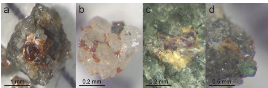
Figure 1. Images of silicate-bearing polycrystalline diamond aggregates from Orapa (a–d, from Mikhail et al. 2019b).
