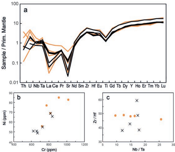
Figure 11. Trace element zonation in three different grains of websteritic garnet in PDA from Venetia (sample V948, Jacob et al. 2000). (a) Spidergrams (normalized to primitive mantle: Sun and McDonough 1989) show significant differences in most elements apart from titanium and the mid and heavy REE in the grains. (b) compatible element Ni and Cr variations ( crosses : grain averages, orange are zones in two different grains), (c) variations in Nb/Ta and Zr/Hf ratios in the zoned grains.
