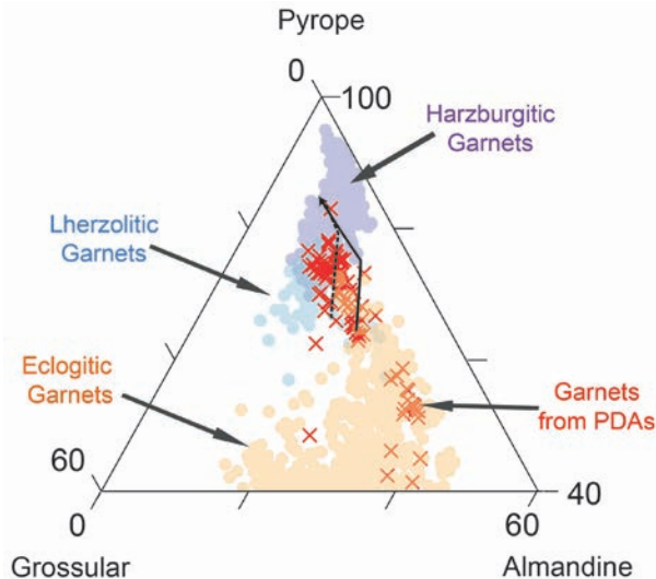
Figure 12. Selected model results for predicted garnet compositions during progressive metasomatism and diamond formation at 5 GPa and 1000 °C. The lines for the runs plotted are thick enough to represent the average trajectories for an eclogitic fluid reacting with model peridotites (lherzolite, harzburgite, and dunite) and model peridotites (lherzolite, harzburgite, and dunite) + aragonite ( dashed line ). Data are from Mikhail et al. (2021) and the input and output files are available at https://doi.org/10.17630/32ebd3c0-bba6-4aa1-9b6d-c53a0a3b61e0 . All comparative data shown are taken from the same sources as listed in the caption of Figure 7c.
