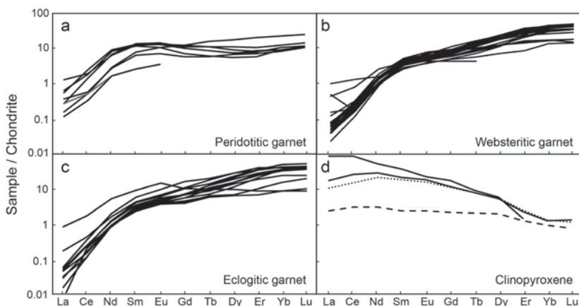
Figure 9. Chondrite-normalised rare earth element (REE) patterns for garnets (a–c) and clinopyroxenes (d) from PDAs. Different signatures in (d) denote peridotitic (solid lines), websteritic (dotted line) and eclogitic (dashed line) clinopyroxenes. Data from Jacob et al. (2000), Dobosi and Kurat (2010), Sobolev et al. (2016), and Mikhail et al. (2019b). Chondrite data from Sun and McDonough (1989).
