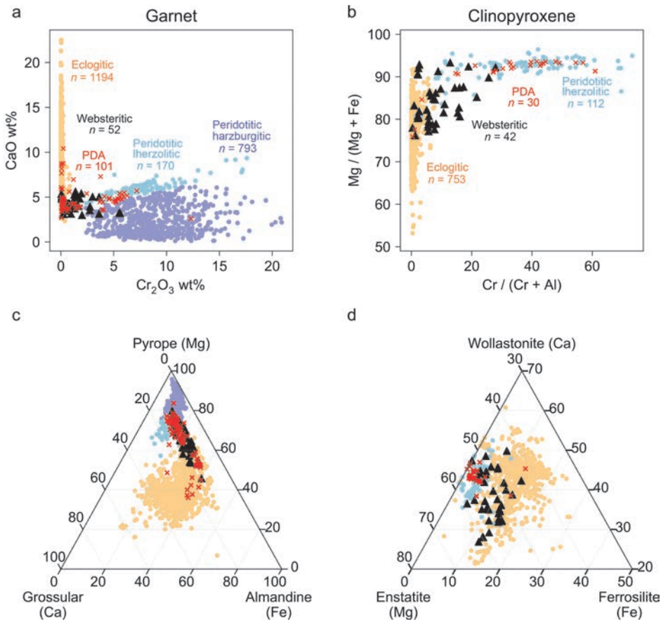
Figure 7. Inclusion parageneses and end-member compositions for garnets and clinopyroxenes from monocrystalline diamond and PDAs. The diamond inclusion database contains geochemical and metadata for > 9000 diamond inclusions. These plots utilize the clinopyroxene ( n = 926 ), and garnet ( n = 2628 ) data from lithospheric mantle diamonds. The data used here are sourced from Stachel and Harris (2008 and references therein) supplemented with more recent datasets (Viljoen et al. 1999; Cartigny et al. 2009; De Stefano et al. 2009; Hunt et al. 2009; Tappert et al. 2009; van Rythoven and Schulze 2009; Bulanova et al. 2010; Miller et al. 2014; Smith et al. 2016; Sobolev et al. 2016; Mikhail et al. 2019a; Jacob et al. unpublished).
