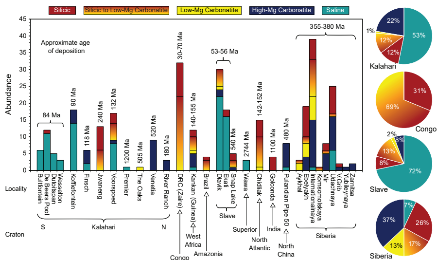
Figure 12. Worldwide abundance and distribution of HDF compositions, separated by locations and cratons. Relative abundances are presented for selected cratons. The database for this figure includes available published sources (Weiss et al. 2022) and data for Bultfontein, Dutoitspan, Wesselton, Premier, The Oaks, River Ranch (Weiss, unpublished data); Venetia (Kempe et al. 2021b); Chidliak (Elazar and Weiss 2021); Golconda (Schrauder 1997) and Pulandian (Mershon et al. 2021). The Kalahari Craton includes the Kaapvaal and Zimbabwe Cratons with the Limpopo Belt between them.
