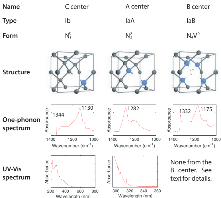
Figure 24. Summary of the nitrogen-related defects which form the basis for the Type I diamond classification. Diamonds which contain a similar concentration of both A and B centers are referred to as Type IaAB or simply Type Ia. Incomplete bonds between atoms indicate that the atoms do not form a bond and are included simply to provide a guide to the eye.
