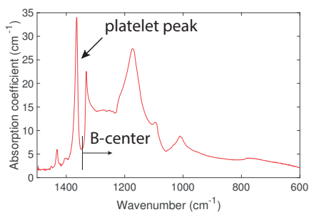
Figure 25. Infrared absorption spectrum of a regular Type IaB diamond, displaying a prominent B' platelet peak at 1365\text{ cm}^{-1} .
