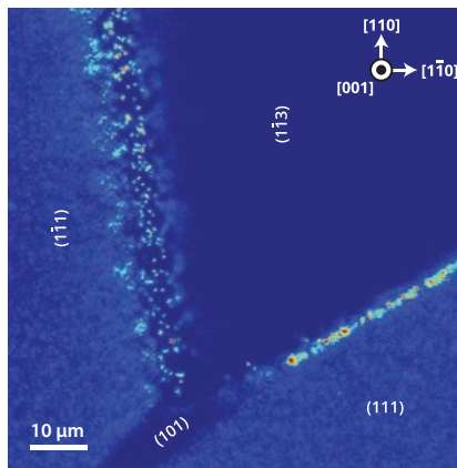
Figure 23. Decoration of growth sector boundaries in an as-grown HPHT sample, as imaged by a single-photon counting fluorescence microscope. The interfaces between each of the labelled growth sectors are decorated with isolated nitrogen-vacancy centers. Each of the bright spots on the (\bar{1}\bar{1}1) \rightarrow (113) transition corresponds to a single atomic nitrogen-vacancy pair, which can be detected with high efficiency using an advanced fluorescence microscope. In this case it is possible to routinely reach ultimate sensitivity i.e., the detection of a single defect. The less bright fluorescence from the \{111\} planes arises from nickel uptake during growth in the \{111\} sectors, but not \{110\} or \{113\} . Modified from Diggle et al. (2020).
