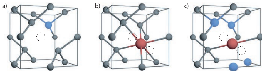
Figure 31. Comparison of the a) NV and b) SiV^- / NiV^- / CoV^- structures. In both cases, only one atom (by number) is missing from the lattice, but in NV the nitrogen remains substitutional, whereas for the larger atoms the impurity relaxes back to a bond-centered location between two lattice sites; the so-called semi-vacancy position. c) The NE8 defect, which emits at 794 nm, is comprised of a nickel atom in the semi-vacancy position with four of its nearest-neighbors replaced by nitrogen (Kupriyanov et al. 1999; Nadolnny et al. 2005).
