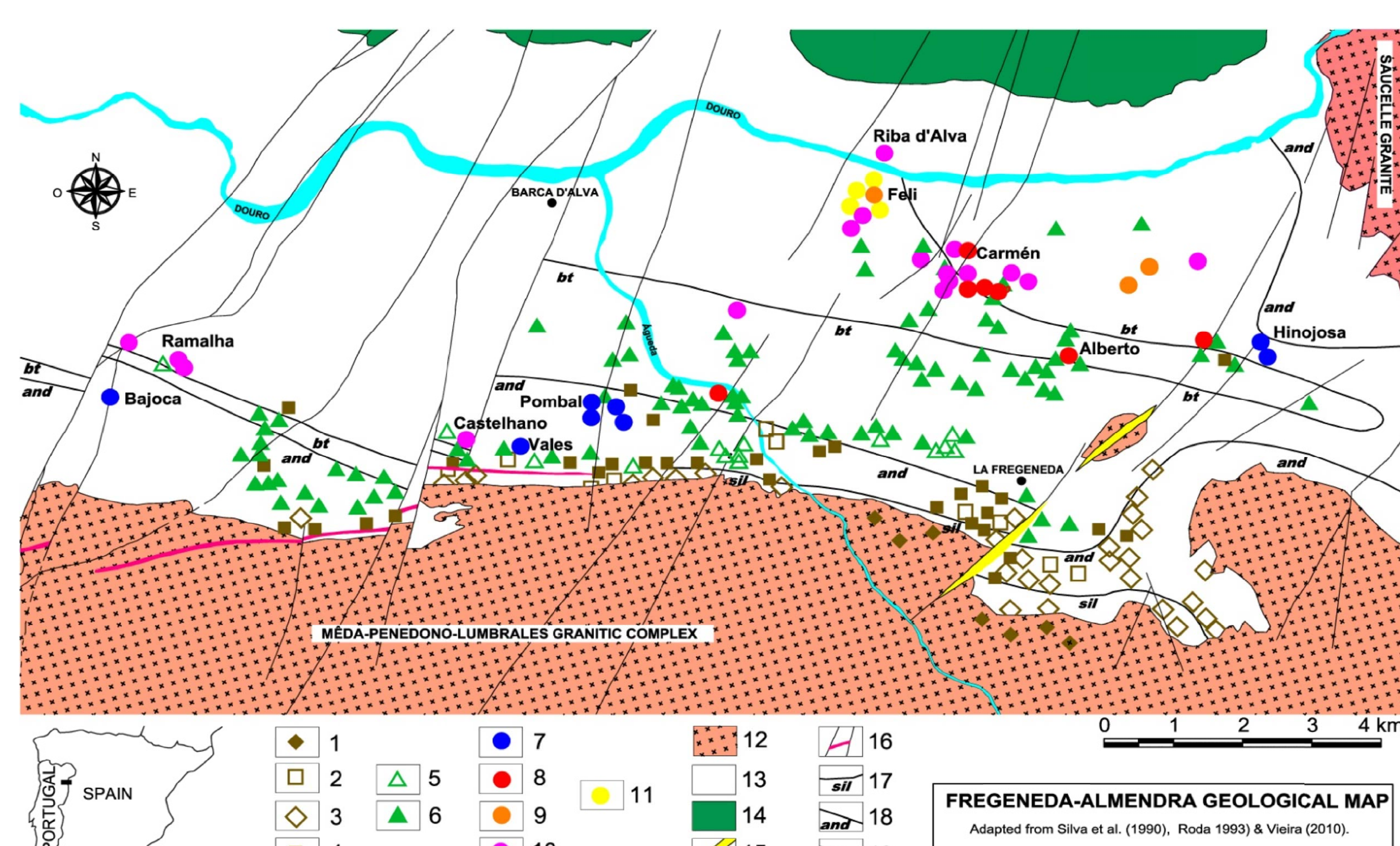
FIGURE 1. Distribution of the pegmatite types in the Fregeneda-Almendra area. Legend: Group i) 1 – simple interior; 2 – quartz + andalusite conformable dykes; 3 – simple dykes and apophyses; 4 – simple conformable; Group ii) 5 – K-feldspar discordant dykes; 6 – simple discordant; Group iii) 7 – petalite-bearing discordant; 8 – spodumene-bearing discordant; 9 – Li-mica + spodumene discordant; 10 – Li-mica-bearing discordant; 11 – Sn-bearing discordant; 12 – syntectonic Variscan granites; 13 – Pre-Ordovician schist-metagreywacke complex; 14 – Ordovician formations; 15 – quartz segregations fractures; 16 – porphyry granitic/riolitic and faults; 17 – sillimanite isograd; 18 – andalusite isograd; 19 – biotite isograd.
