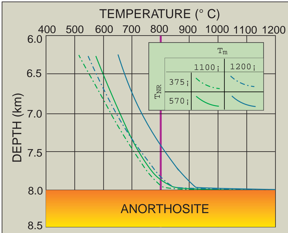
Figure 7. Results of one-dimensional finite difference models for vertical heat loss above an intrusion emplaced at 8 to 13 km. Note that only high magmatic temperature ( T_m = 1200\text{ }^\circ\text{C} ) and high regional geotherm ( > 70\text{ }^\circ\text{C/km} ) produce aureole temperatures > 800\text{ }^\circ\text{C} more than 200 m from the contact. Temperatures plotted are peak temperatures reached at a particular node during conductive heating.
